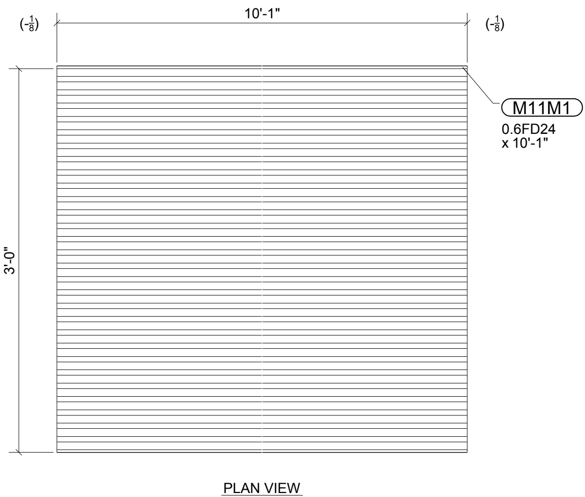
ONE - 24 GA 9/16" FORM DECK - M11M1
