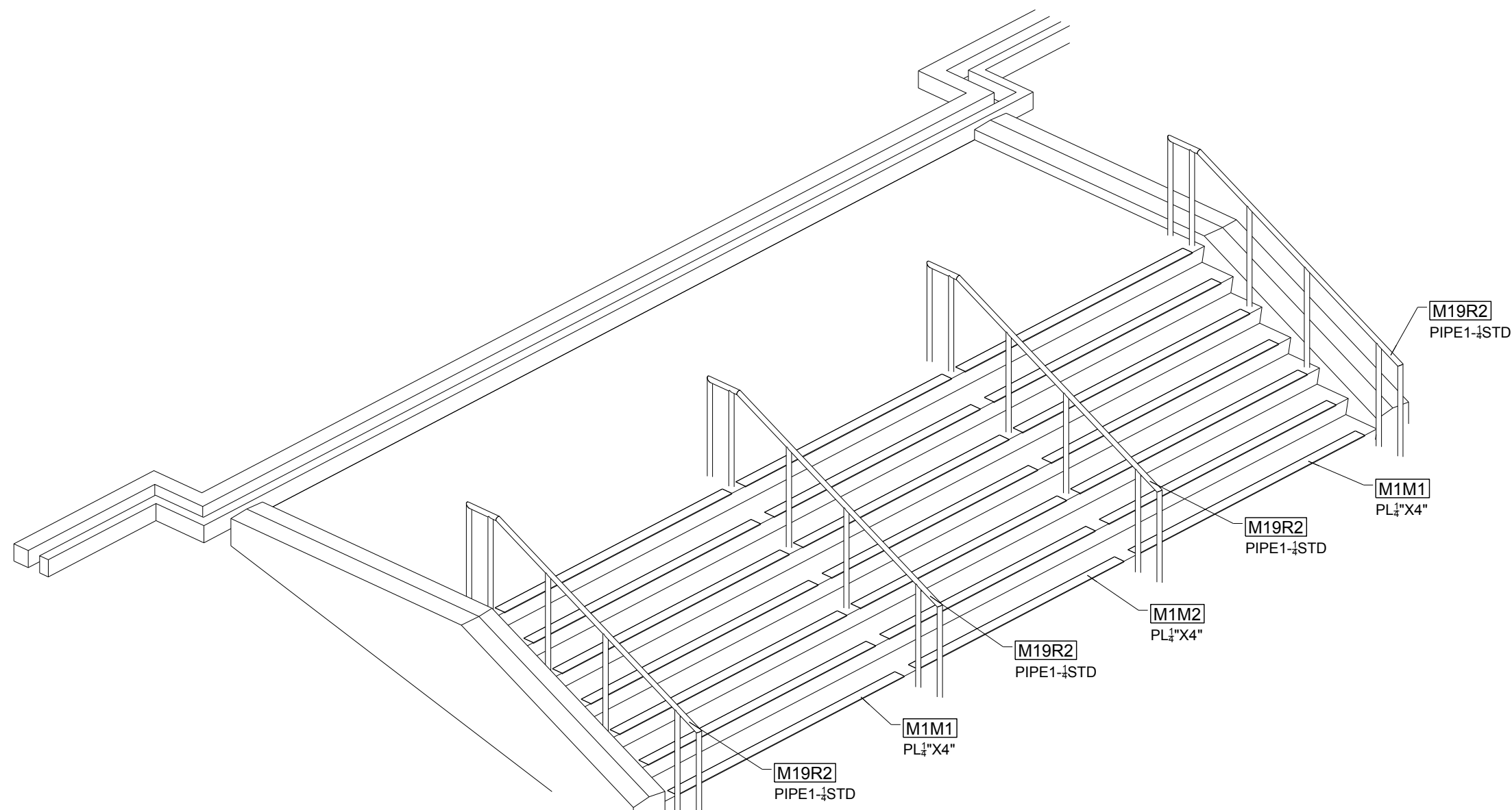
ENTRY STAIR 3D VIEW
