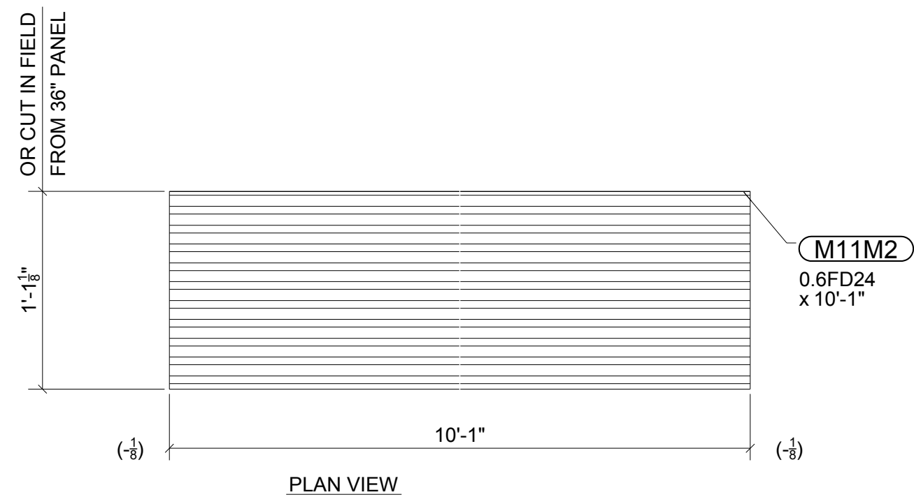
ONE - 24 GA 9/16" FORM DECK - M11M2
