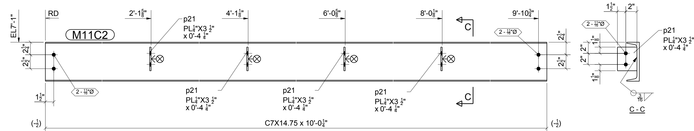
ONE - CHANNEL - M11C2
