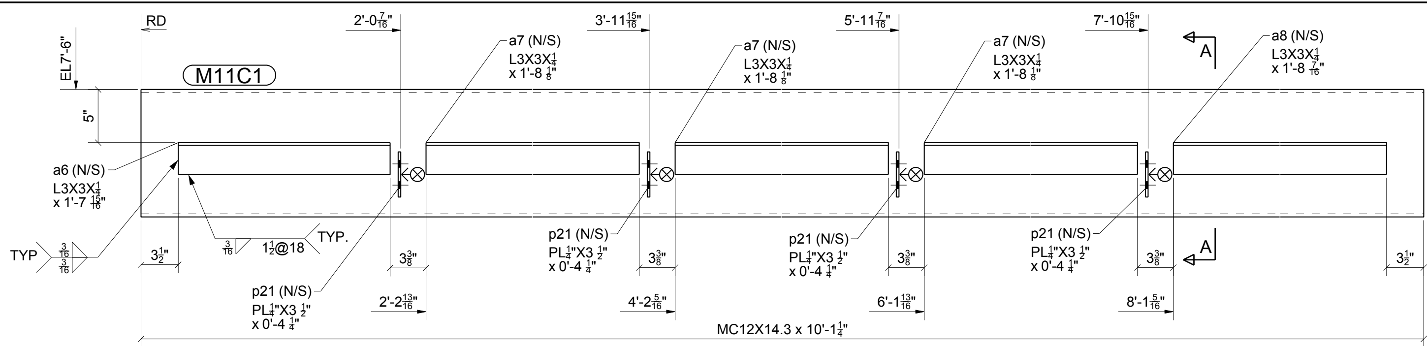
ONE - CHANNEL - M11C1
