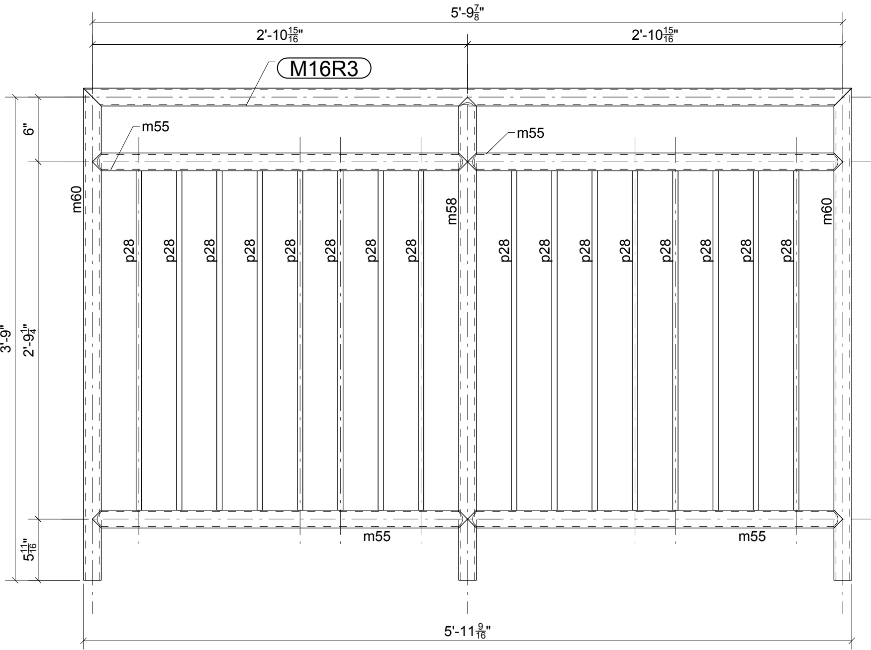
ONE - STAIR 1 GUARDRAIL - M16R3
