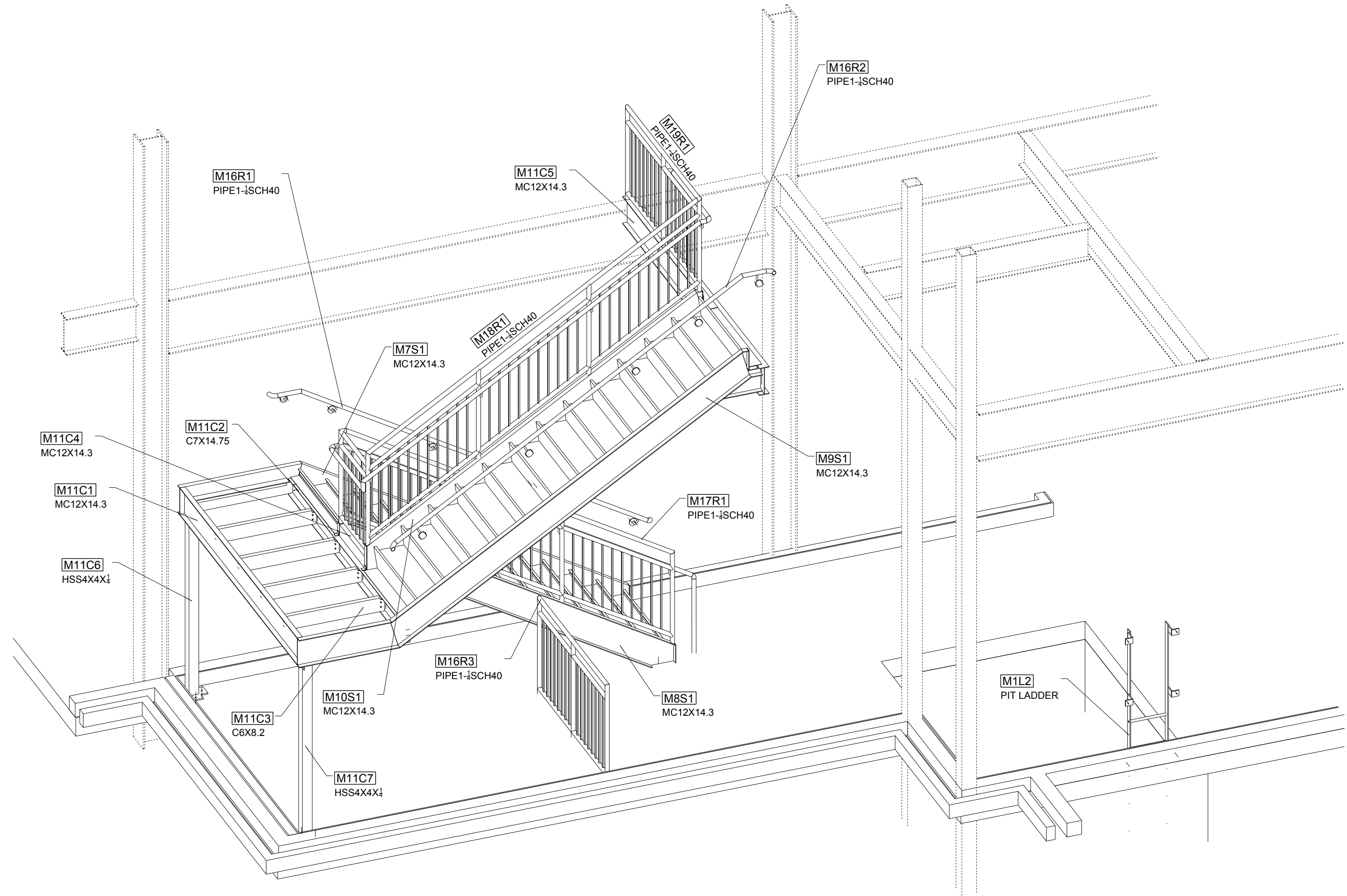
STAIR 1 3D VIEW
