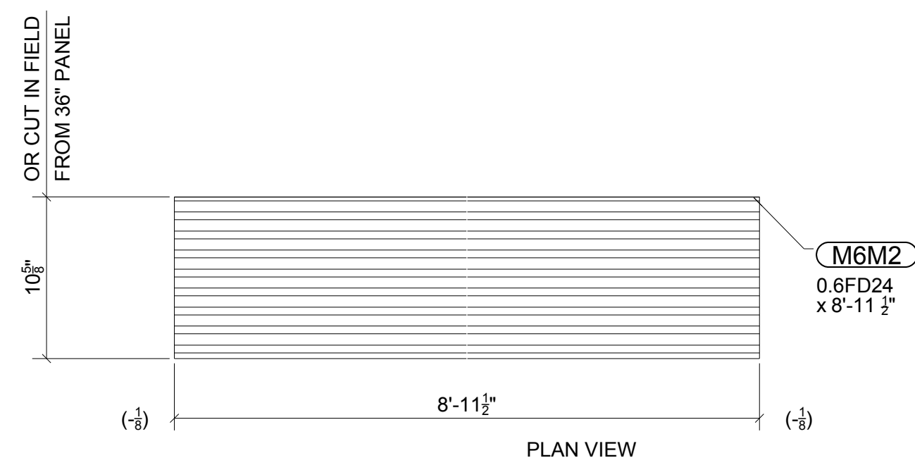
ONE - 24 GA 9/16" FORM DECK - M6M2
