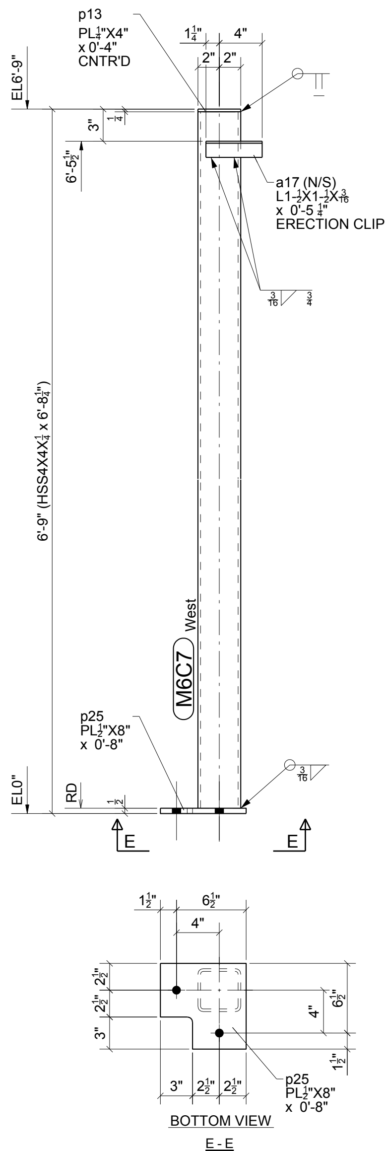
ONE - COLUMN - M6C7
