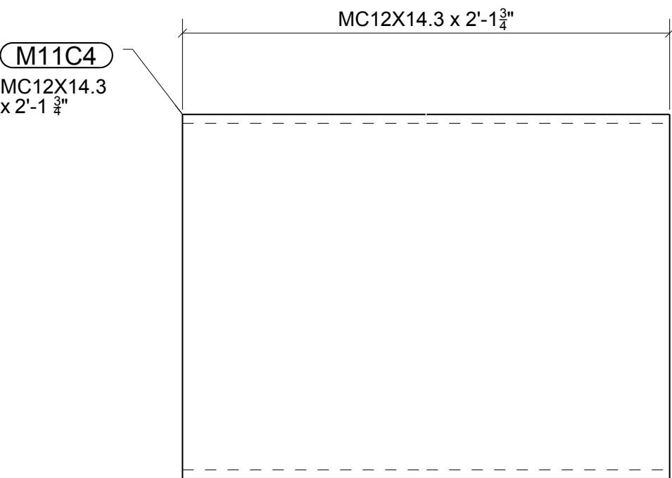
ONE - CHANNEL - M11C4
