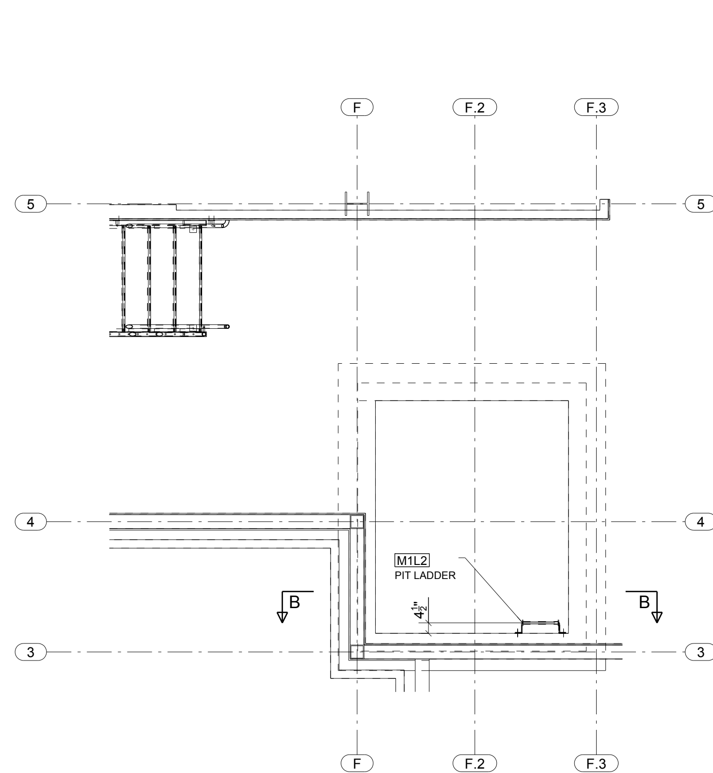
ELEVATOR PIT PLAN
