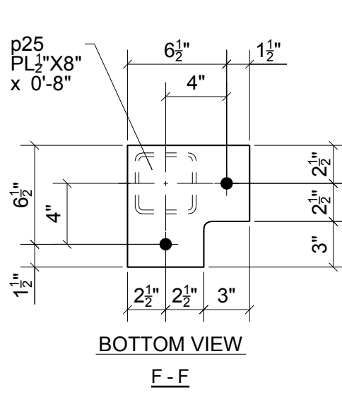
ONE - COLUMN - M11C7
