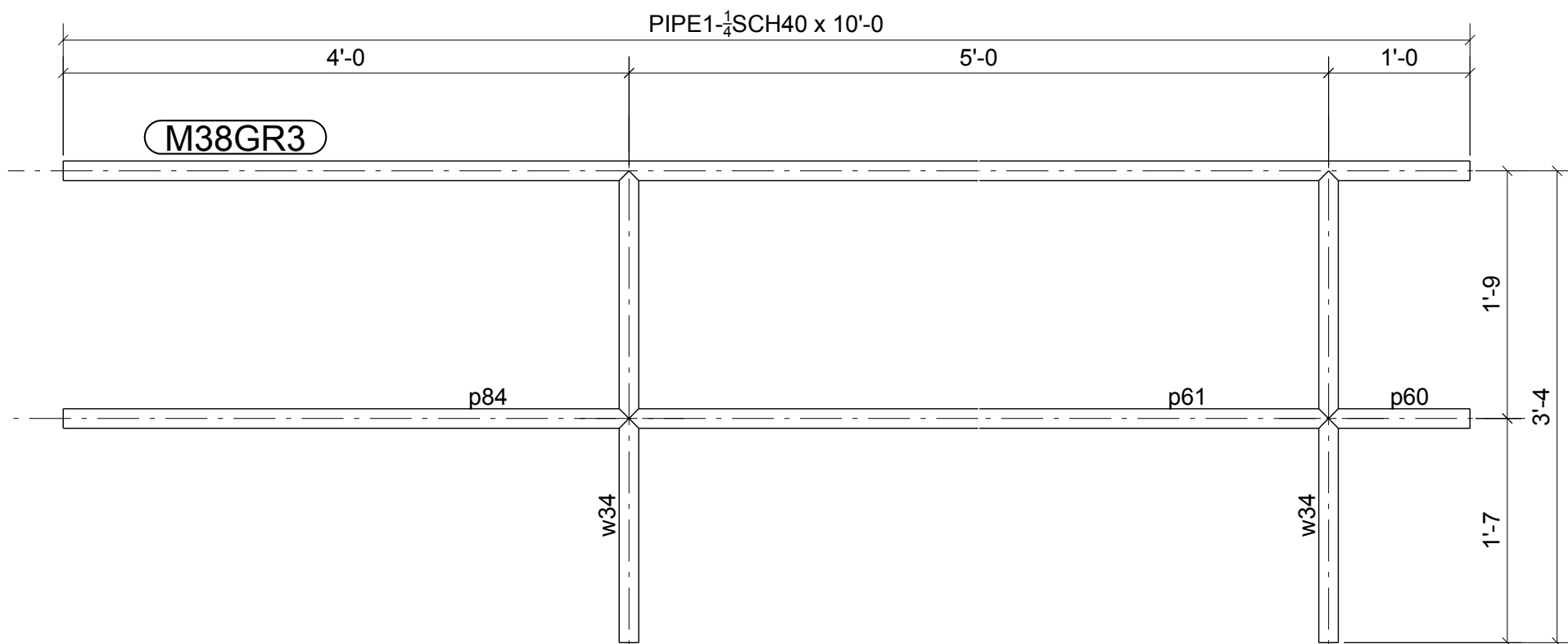
ONE - GUARDRAIL - M38GR3
