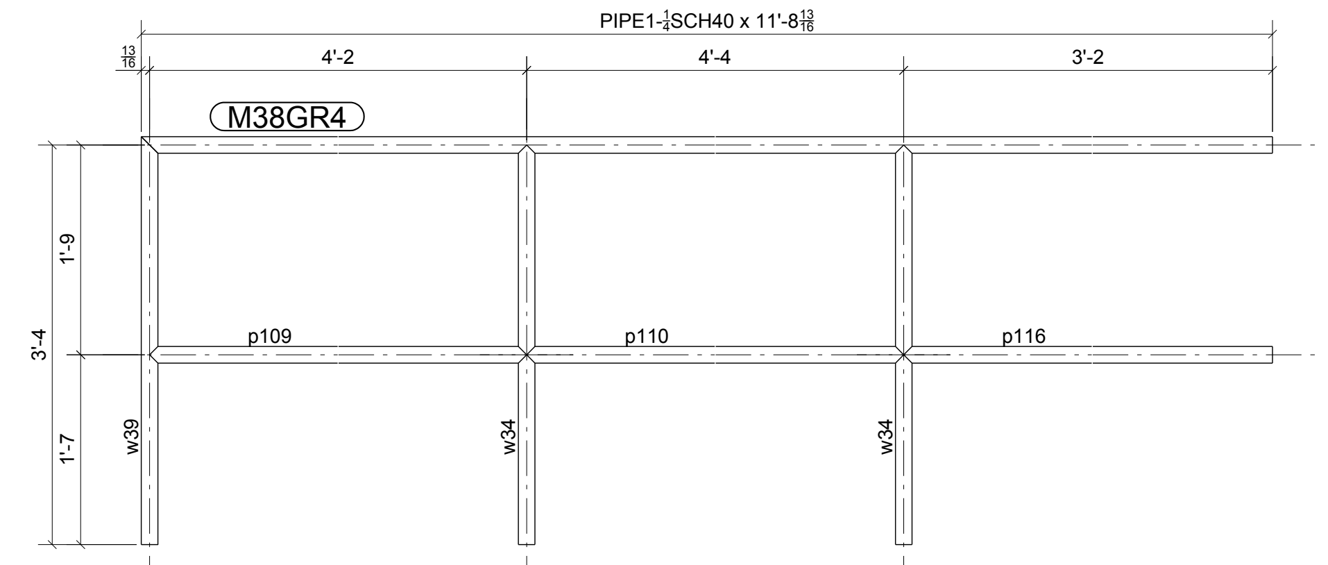
ONE - GUARDRAIL - M38GR4
