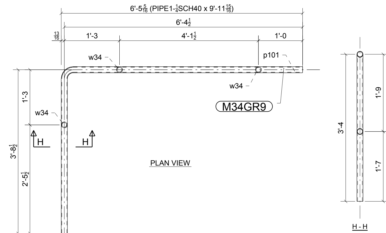
ONE - GUARDRAIL - M34GR9
