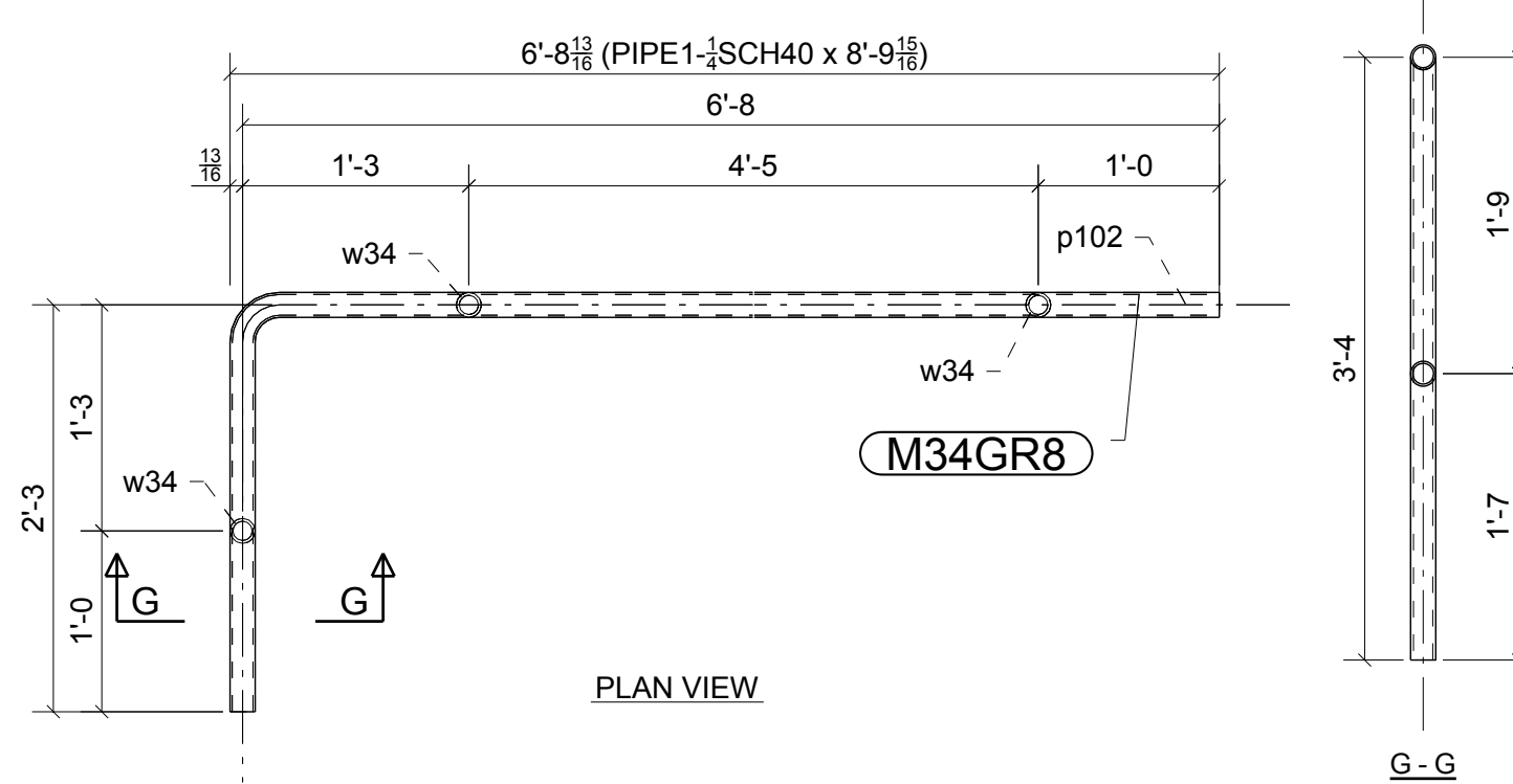
ONE - GUARDRAIL - M34GR8
