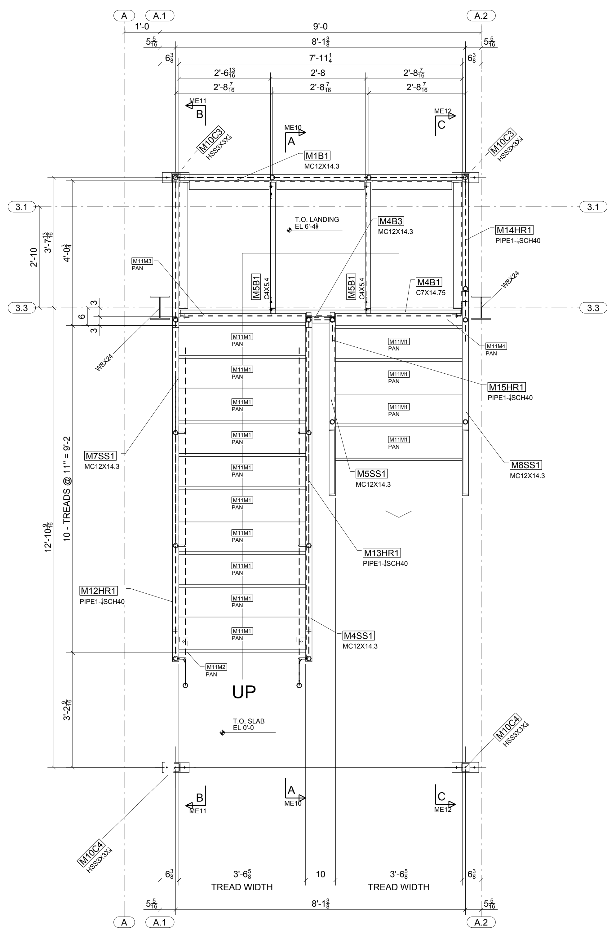
STAIR 1 - GROUND LEVEL TO MID-LANDING 1
