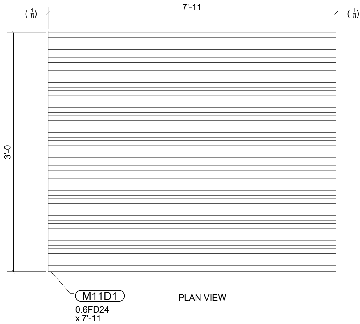
4 - 24 GA 9/16" FORM DECKS - M11D1
