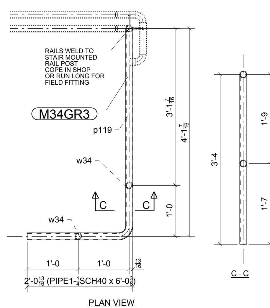
ONE - GUARDRAIL - M34GR3
