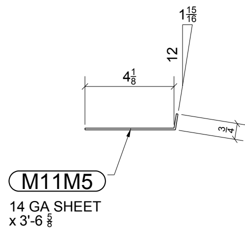
2 - TREADS - M11M5
