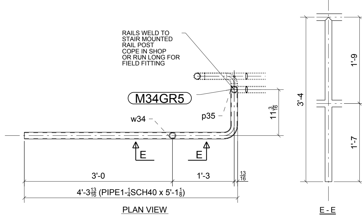
ONE - GUARDRAIL - M34GR5
