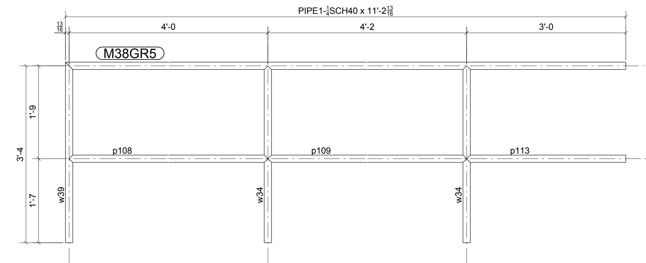
ONE - GUARDRAIL - M38GR5
