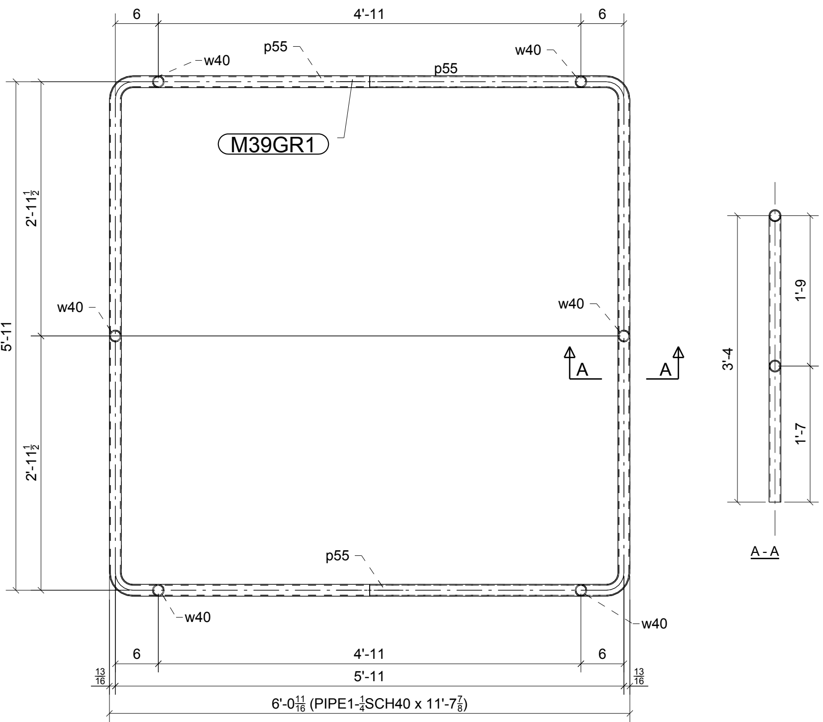
ONE - GUARDRAIL - M39GR1
