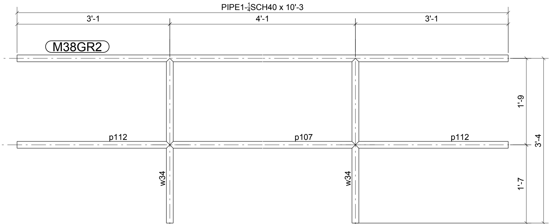
ONE - GUARDRAIL - M38GR2
