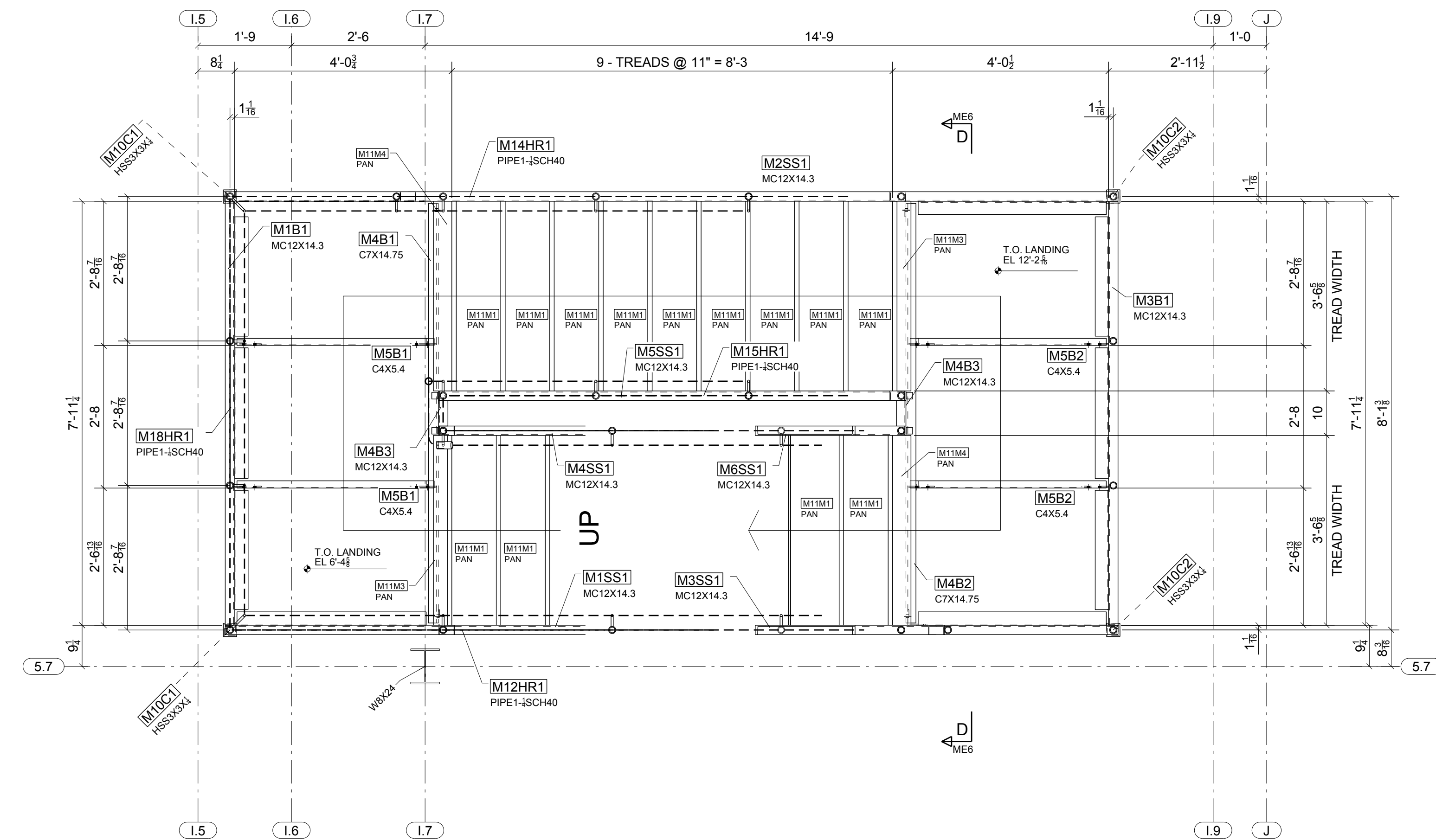
STAIR 3 - MID-LANDING 1 TO MID-LANDING 2
