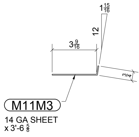
4 - TREADS - M11M3
