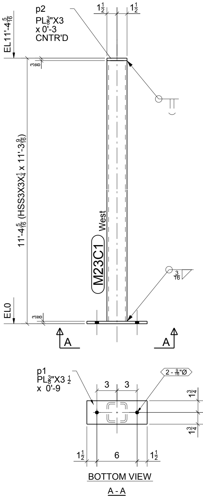
2 - POSTS - M23C1
