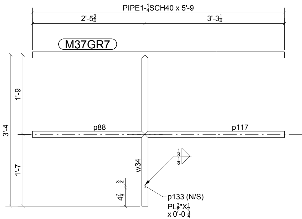
ONE - GUARDRAIL - M37GR7
