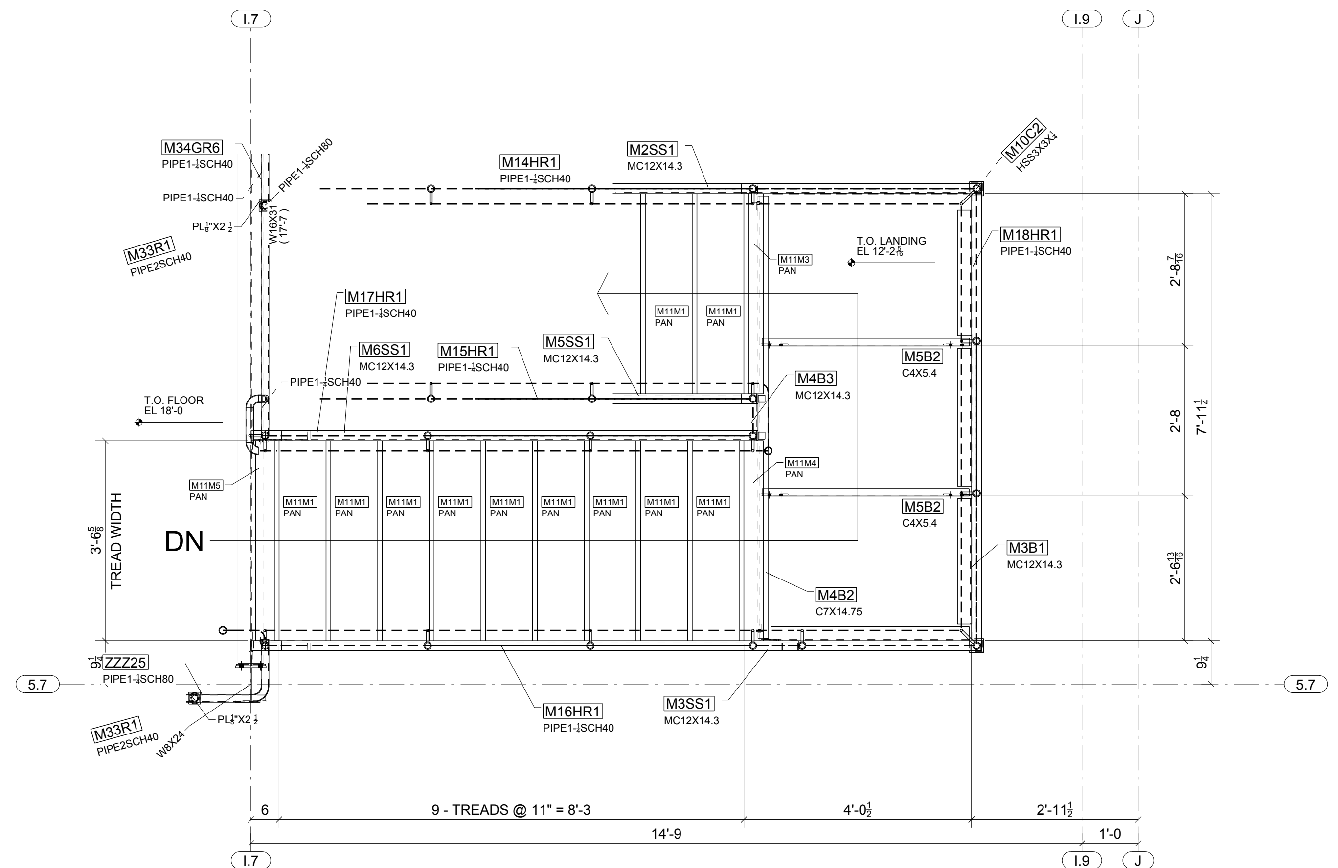
STAIR 3 - MID-LANDING 2 TO MEZZANINE LEVEL
