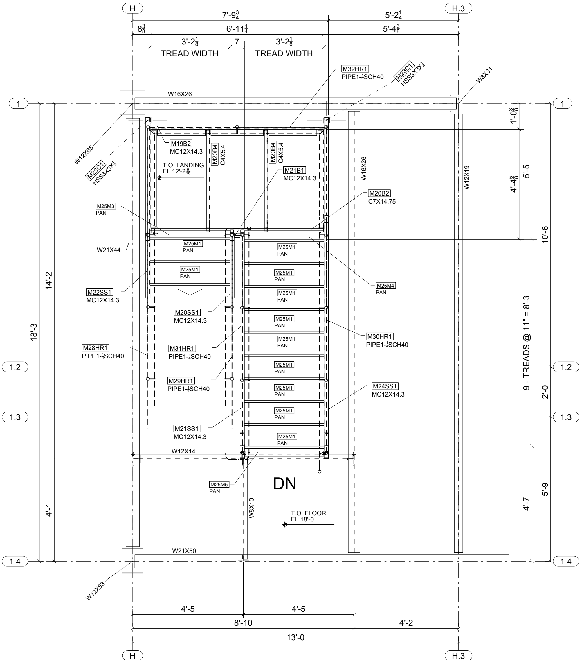
STAIR 2 - MID-LANDING 2 TO MEZZANINE LEVEL
