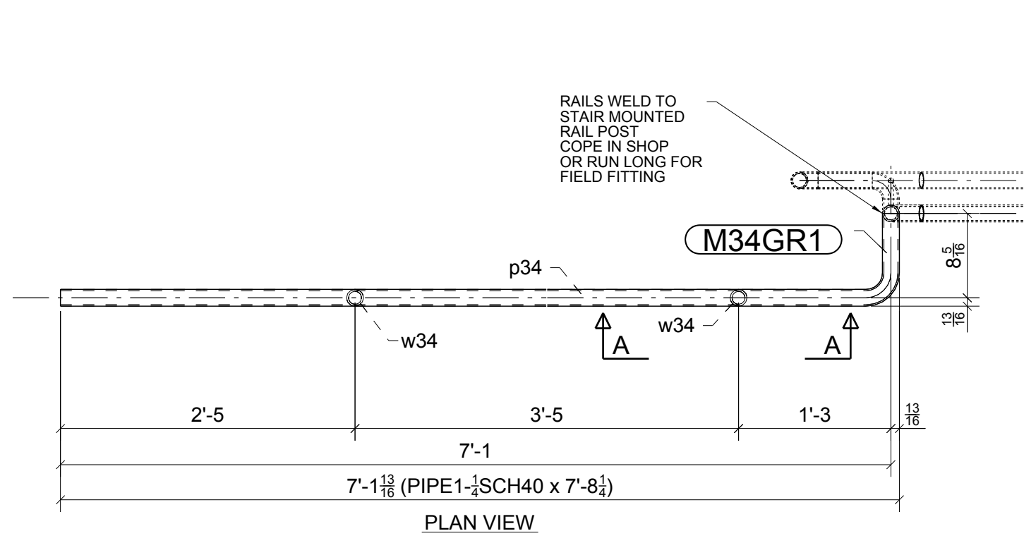
ONE - GUARDRAIL - M34GR1
