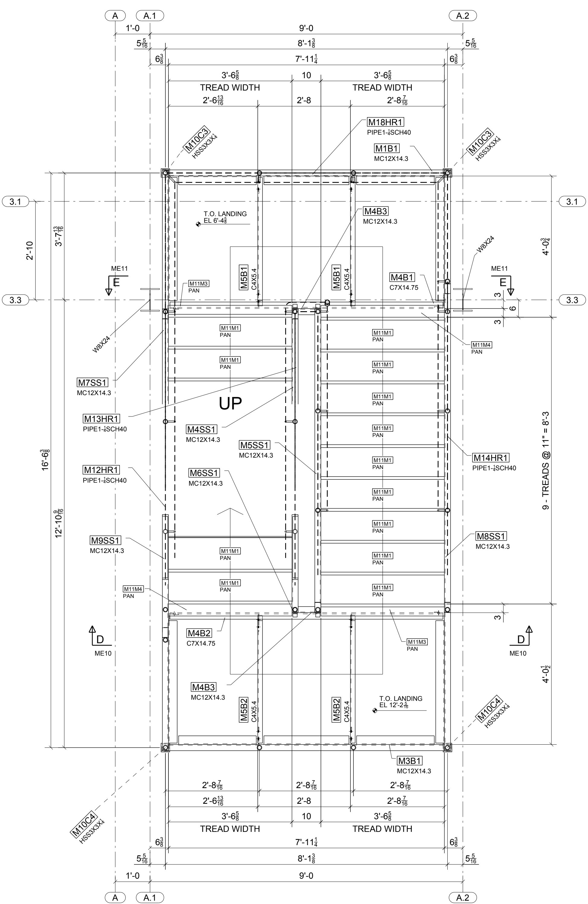
STAIR 1 - MID-LANDING 1 TO MID-LANDING 2
