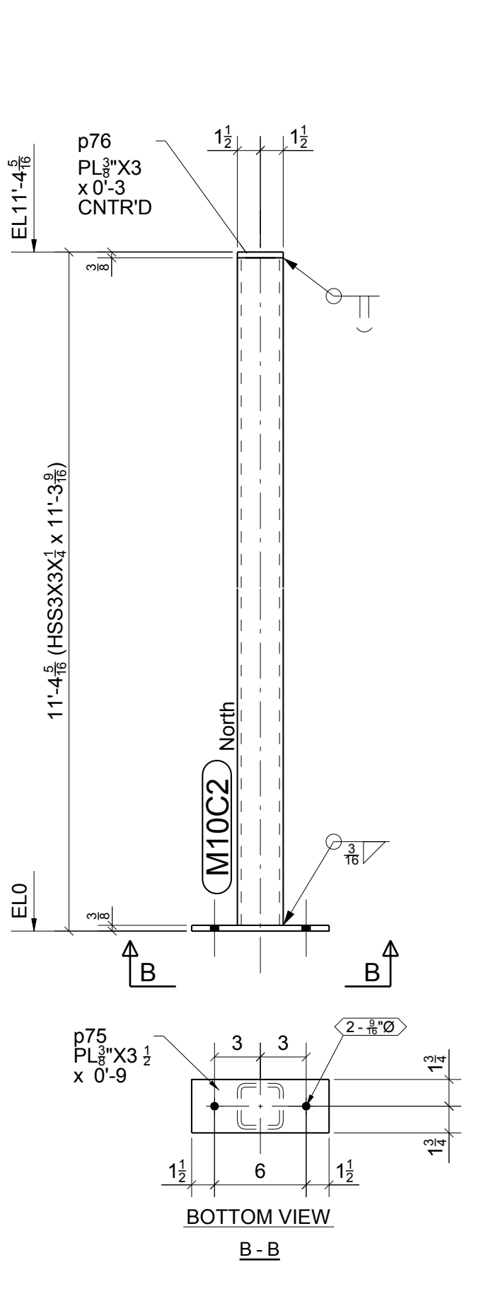
2 - POSTS - M10C2
