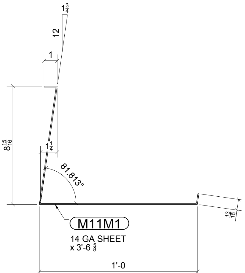
56 - TREADS - M11M1
