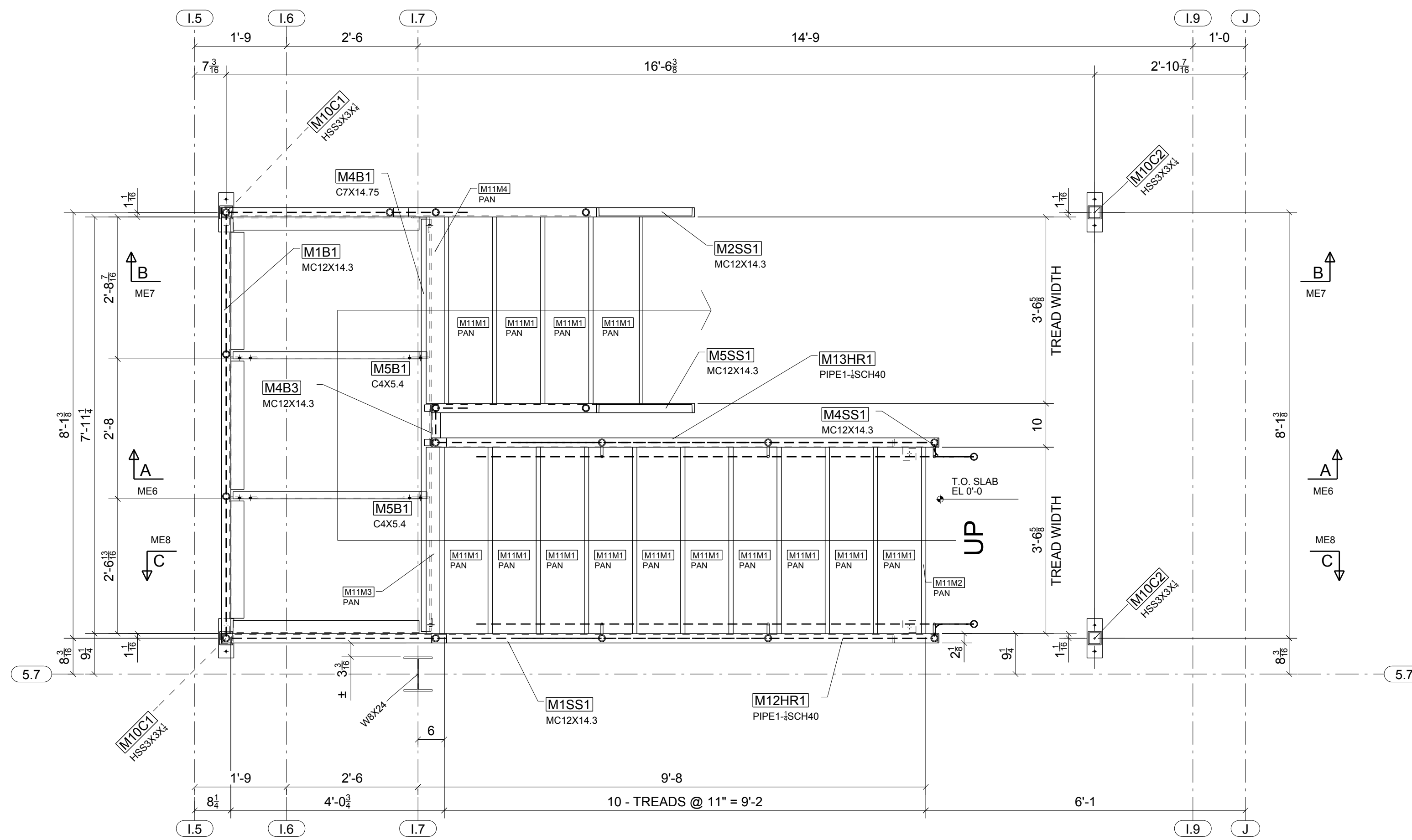
STAIR 3 - GROUND LEVEL TO MID-LANDING 1
