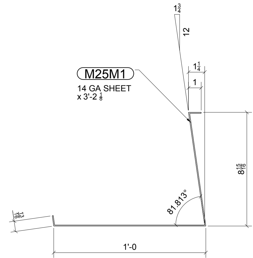
28 - TREADS - M25M1
