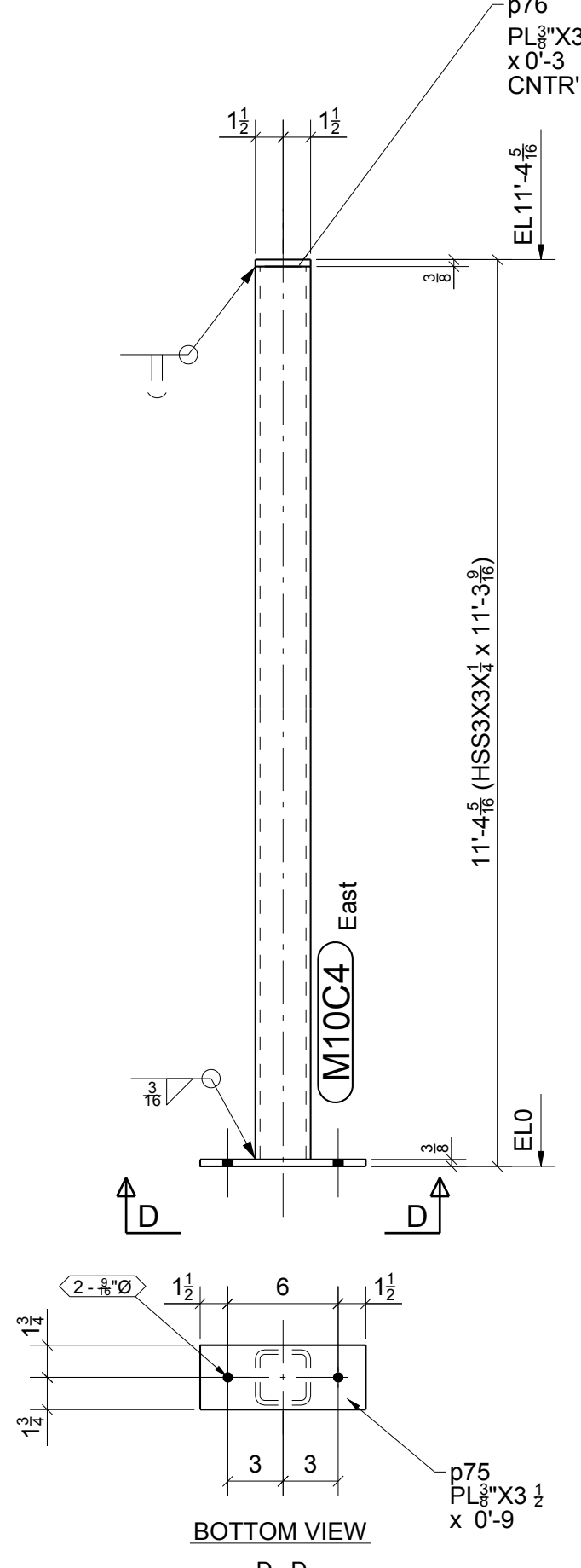
2 - POSTS - M10C4
