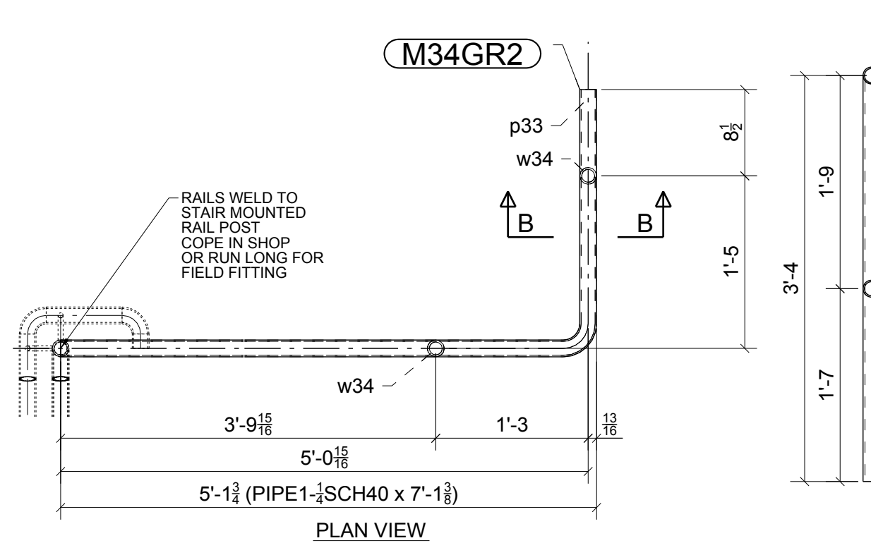
ONE - GUARDRAIL - M34GR2
