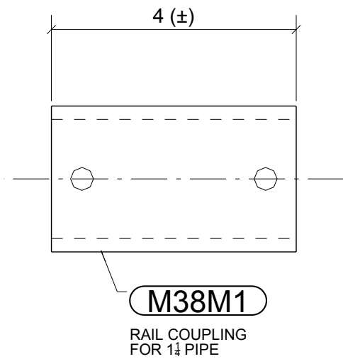
54 - RAIL COUPLINGS - M38M1
