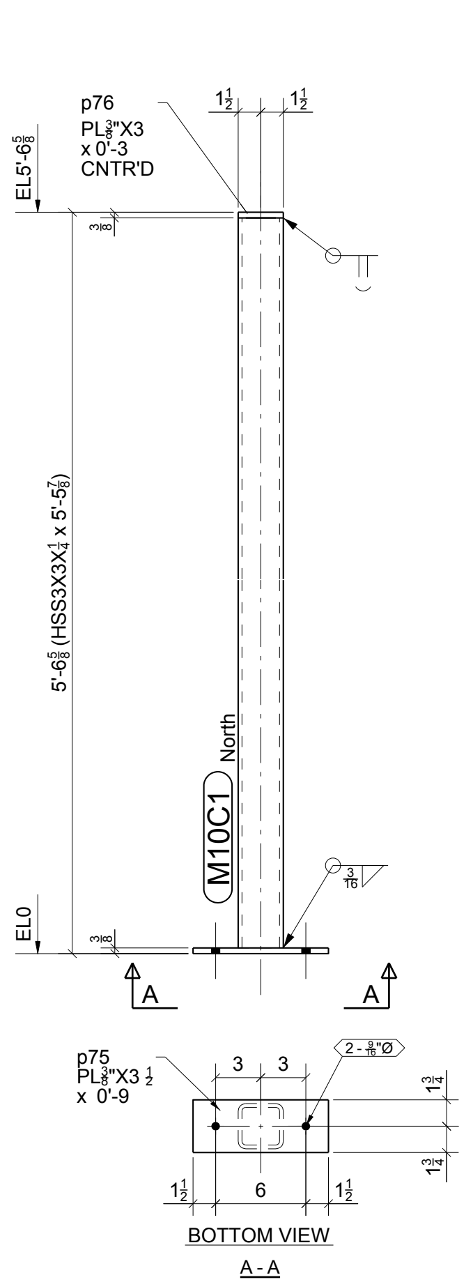
2 - POSTS - M10C1
