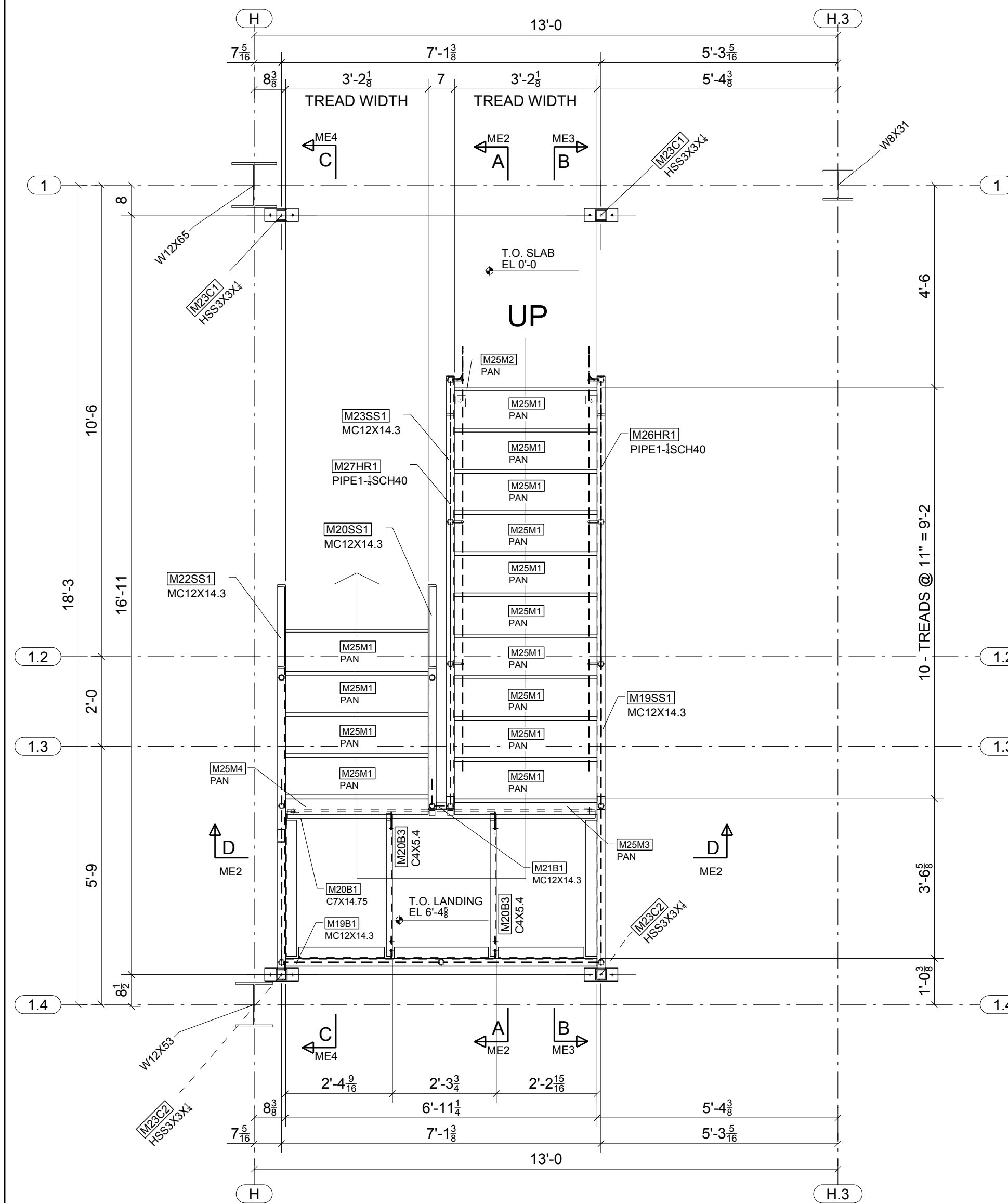
STAIR 2 - GROUND LEVEL TO MID-LANDING 1
