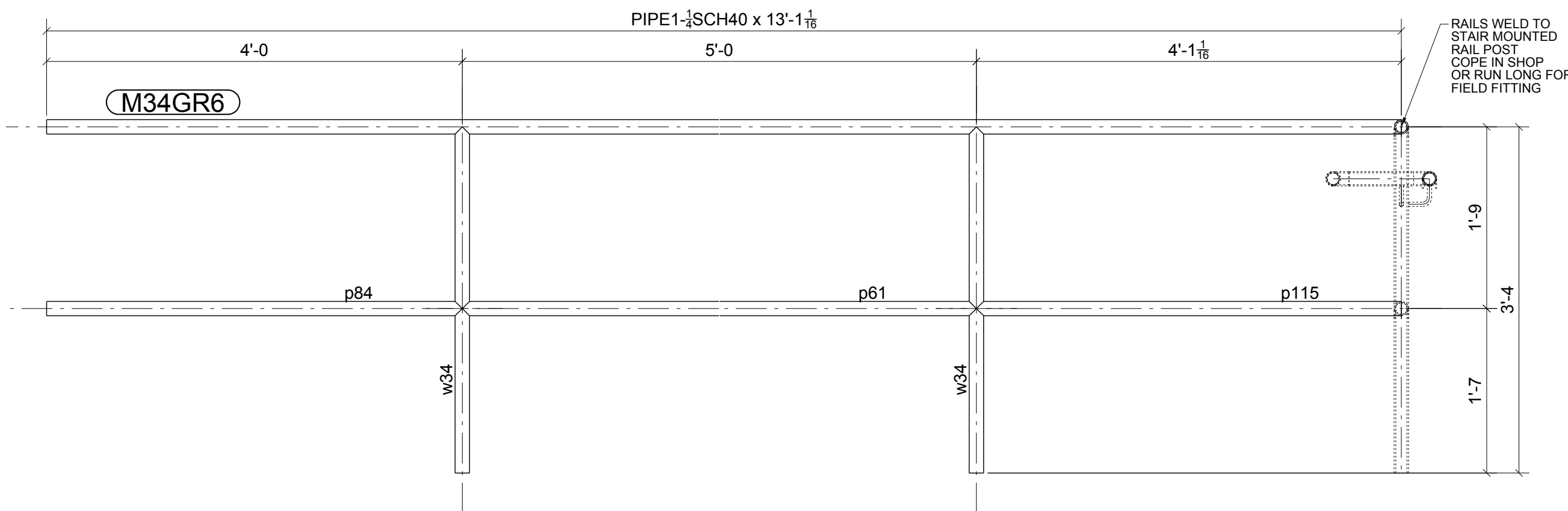
ONE - GUARDRAIL - M34GR6
