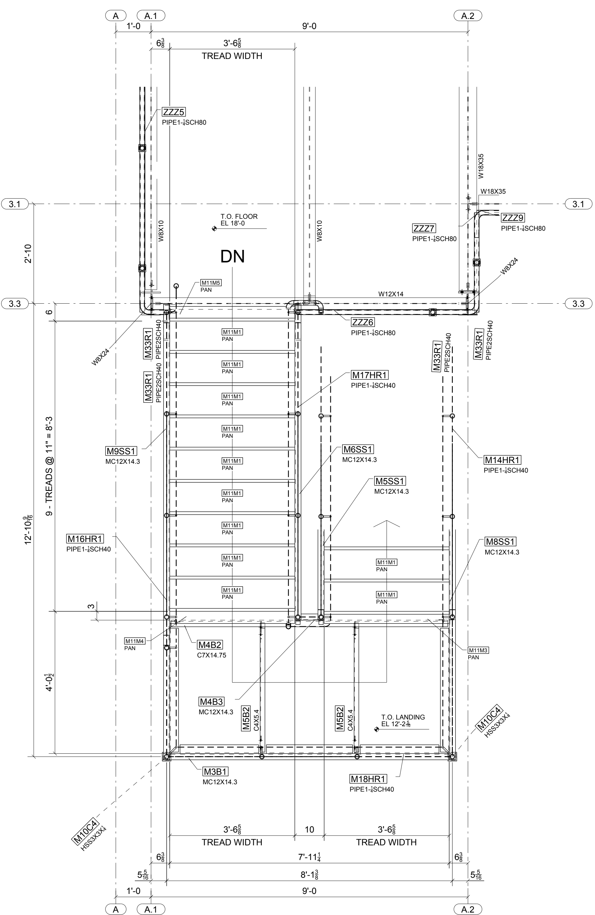
STAIR 1 - MID-LANDING 2 TO MEZZANINE LEVEL
