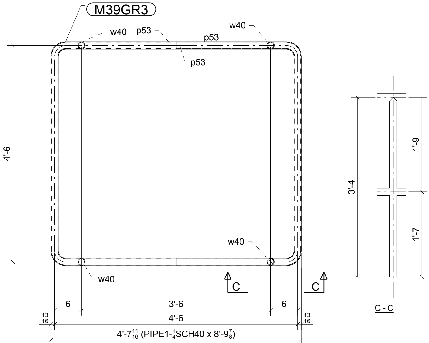
ONE - GUARDRAIL - M39GR3
