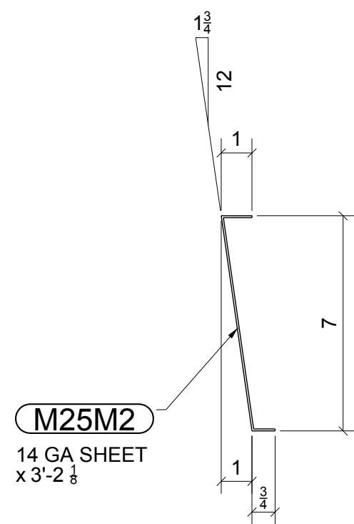
ONE - TREAD - M25M2
