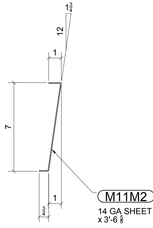
2 - TREADS - M11M2
