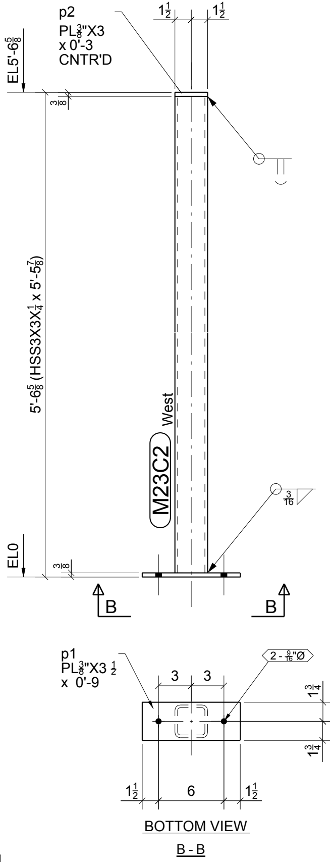
2 - POSTS - M23C2
