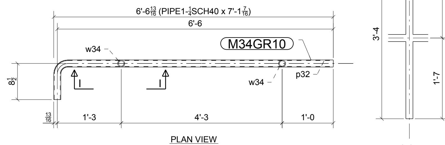
ONE - GUARDRAIL - M34GR10
