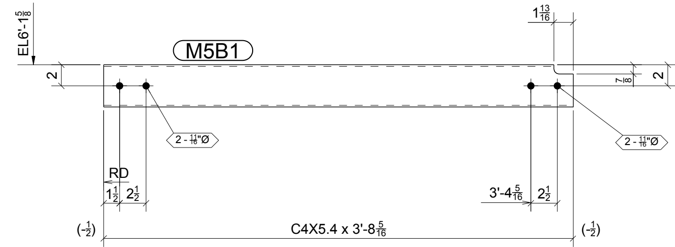
4 - CHANNELS - M5B1
