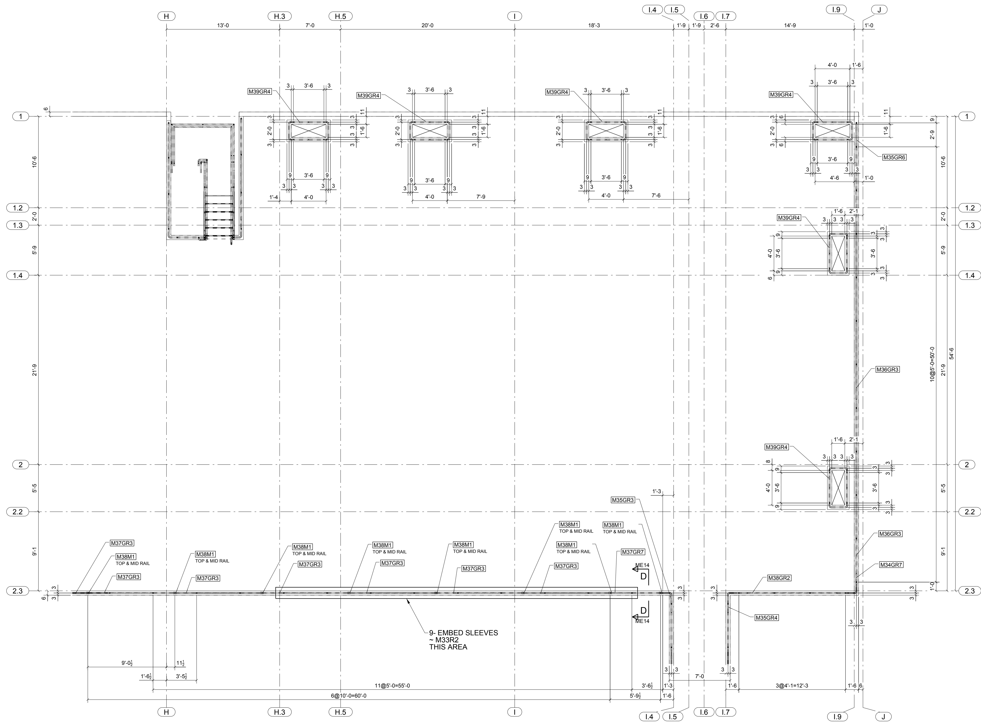
PLATFORM GUARDRAIL PLAN
