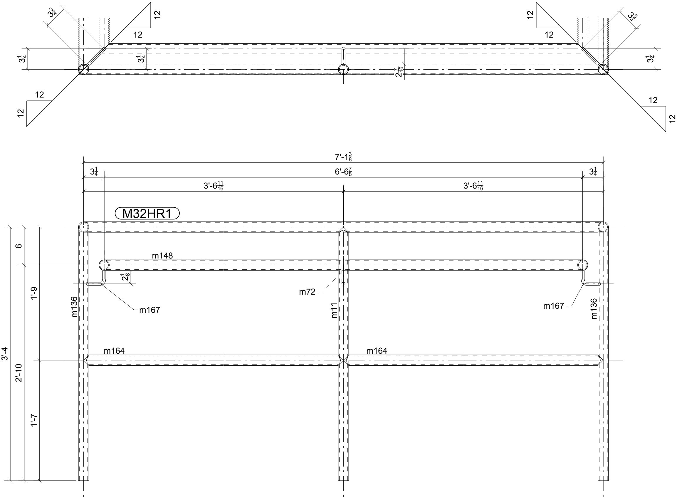
2 - RAILS - M32HR1
