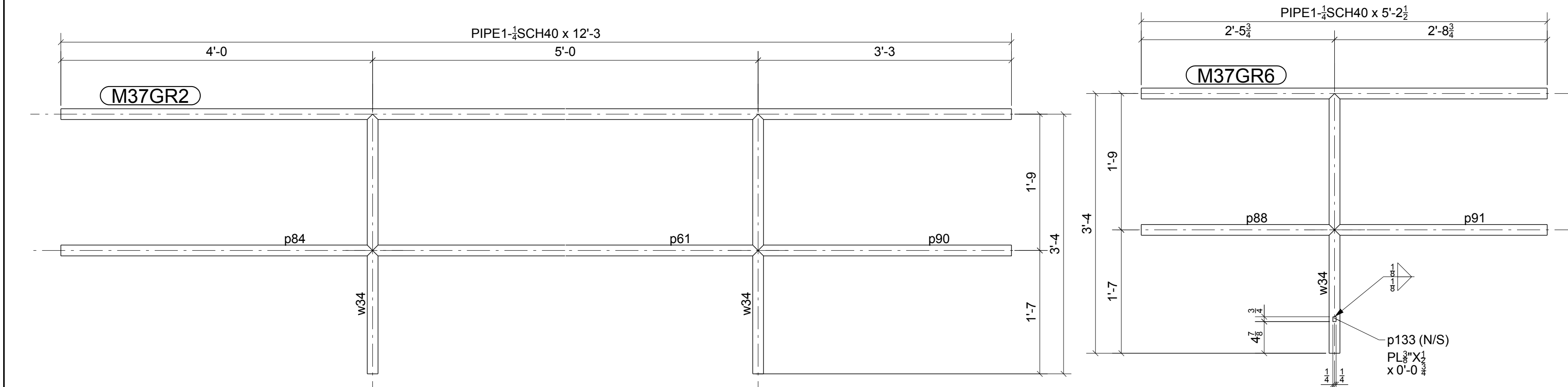
ONE - GUARDRAIL - M37GR2
