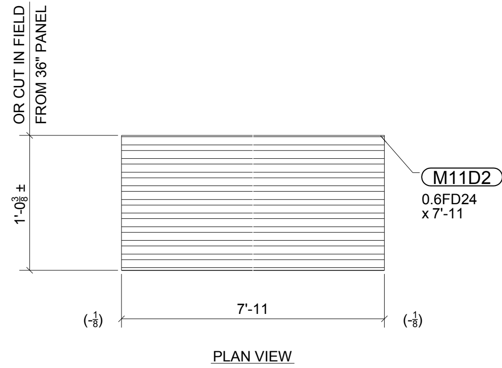
2 - 24 GA 9/16" FORM DECKS - M11D2
