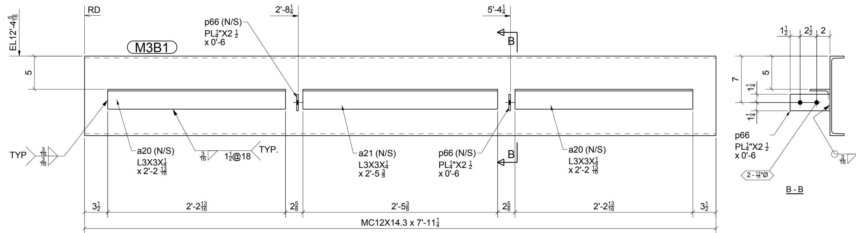
2 - BEAMS - M3B1
