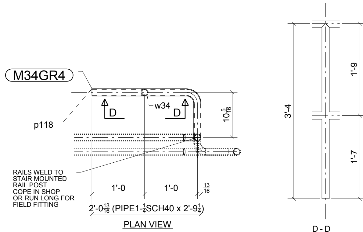
ONE - GUARDRAIL - M34GR4
