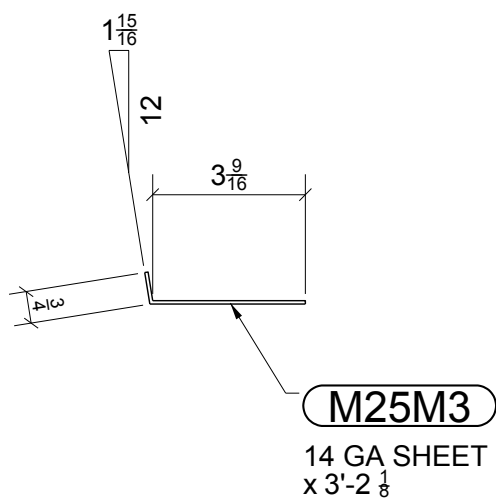
2 - TREADS - M25M3
