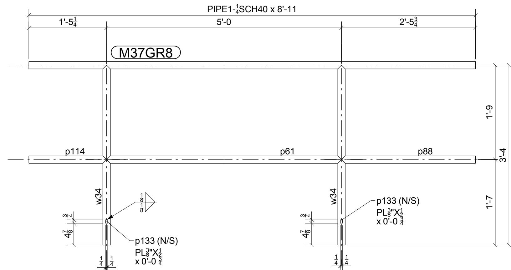
ONE - GUARDRAIL - M37GR8
