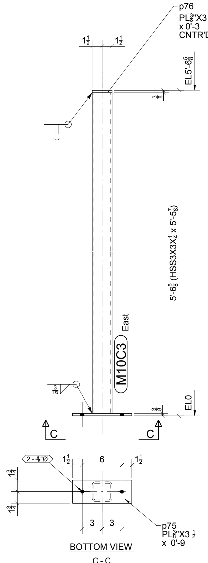
2 - POSTS - M10C3
