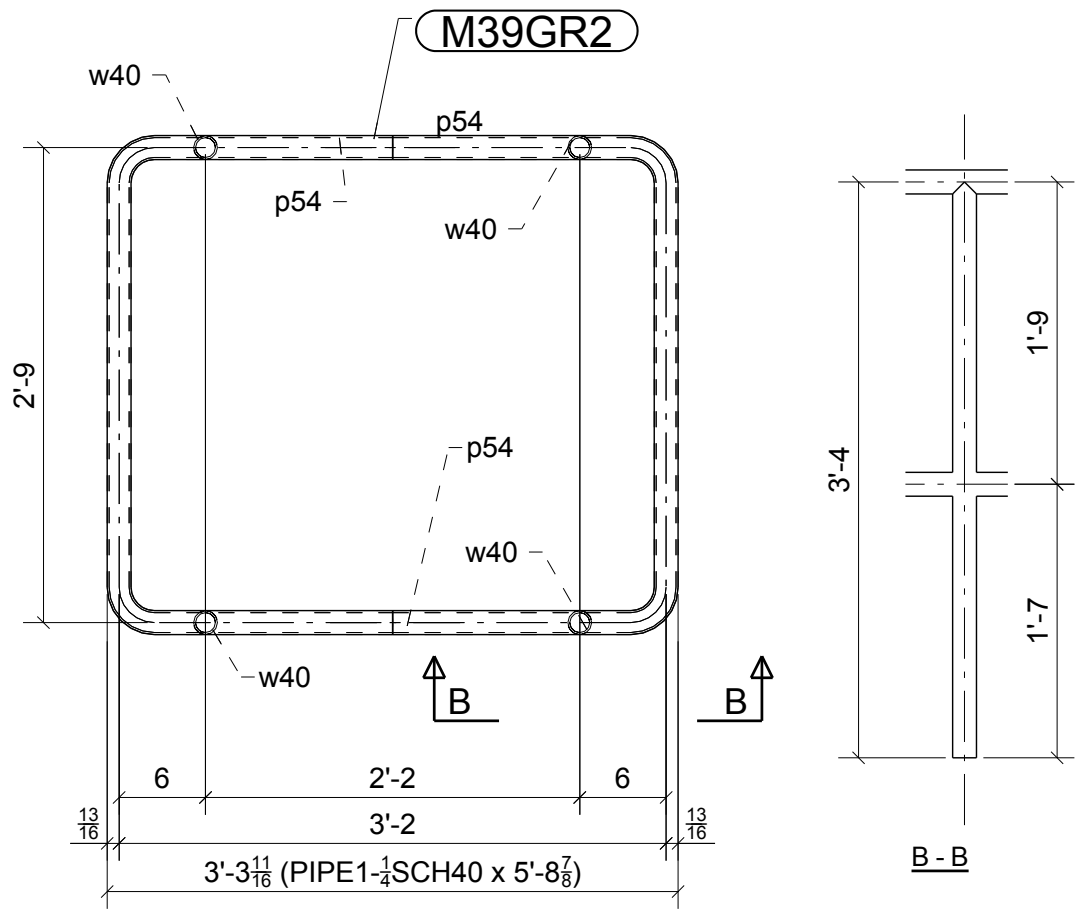
ONE - GUARDRAIL - M39GR2
