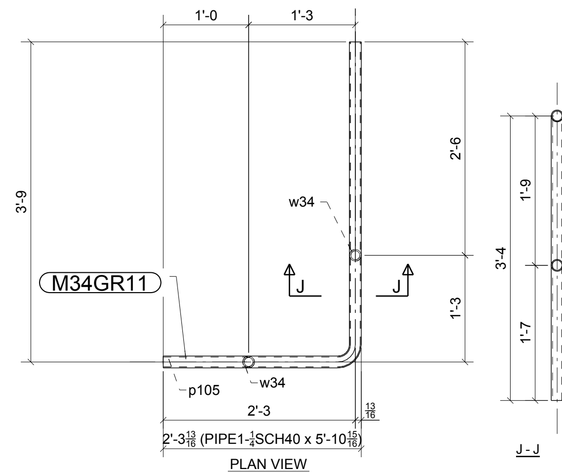
ONE - GUARDRAIL - M34GR11
