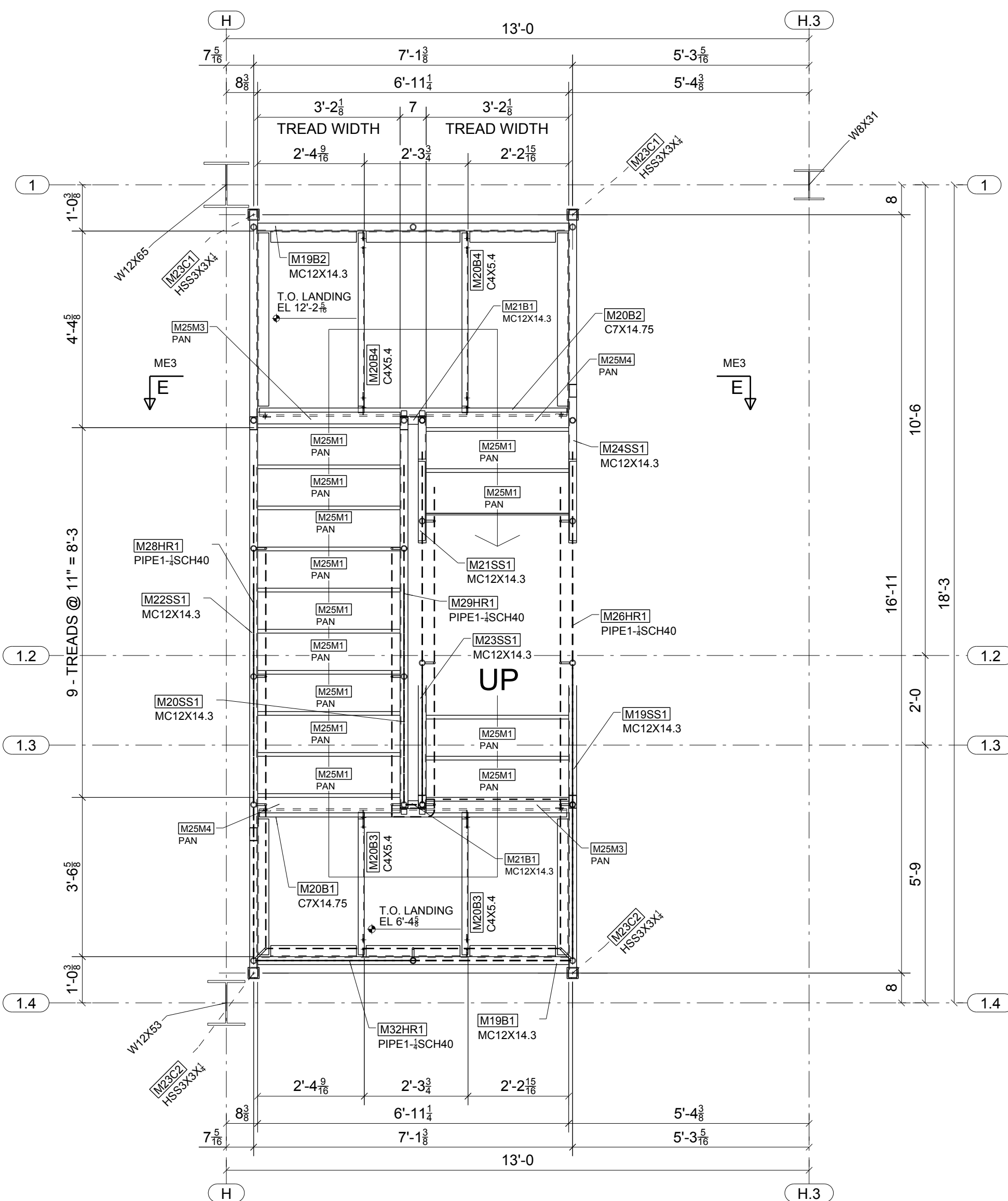
STAIR 2 - MID-LANDING 1 TO MID-LANDING 2
