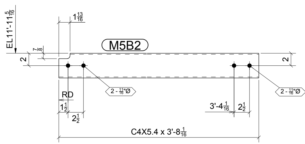
4 - CHANNELS - M5B2
