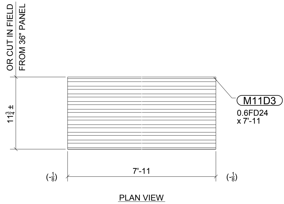
2 - 24 GA 9/16" FORM DECKS - M11D3
