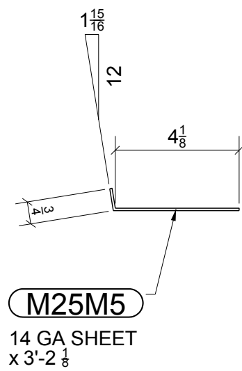
ONE - TREAD - M25M5
