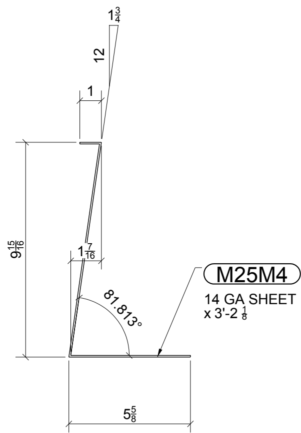
2 - TREADS - M25M4
