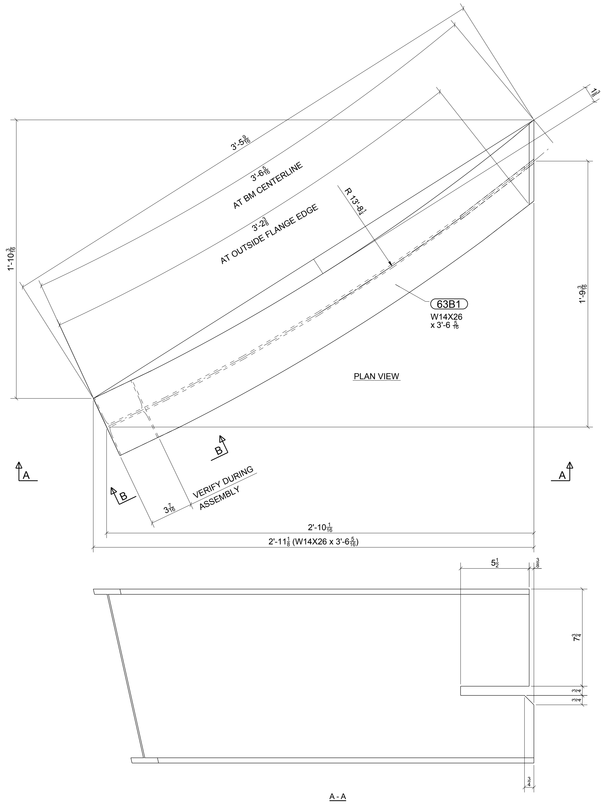
ONE - STRINGER - 63B1
