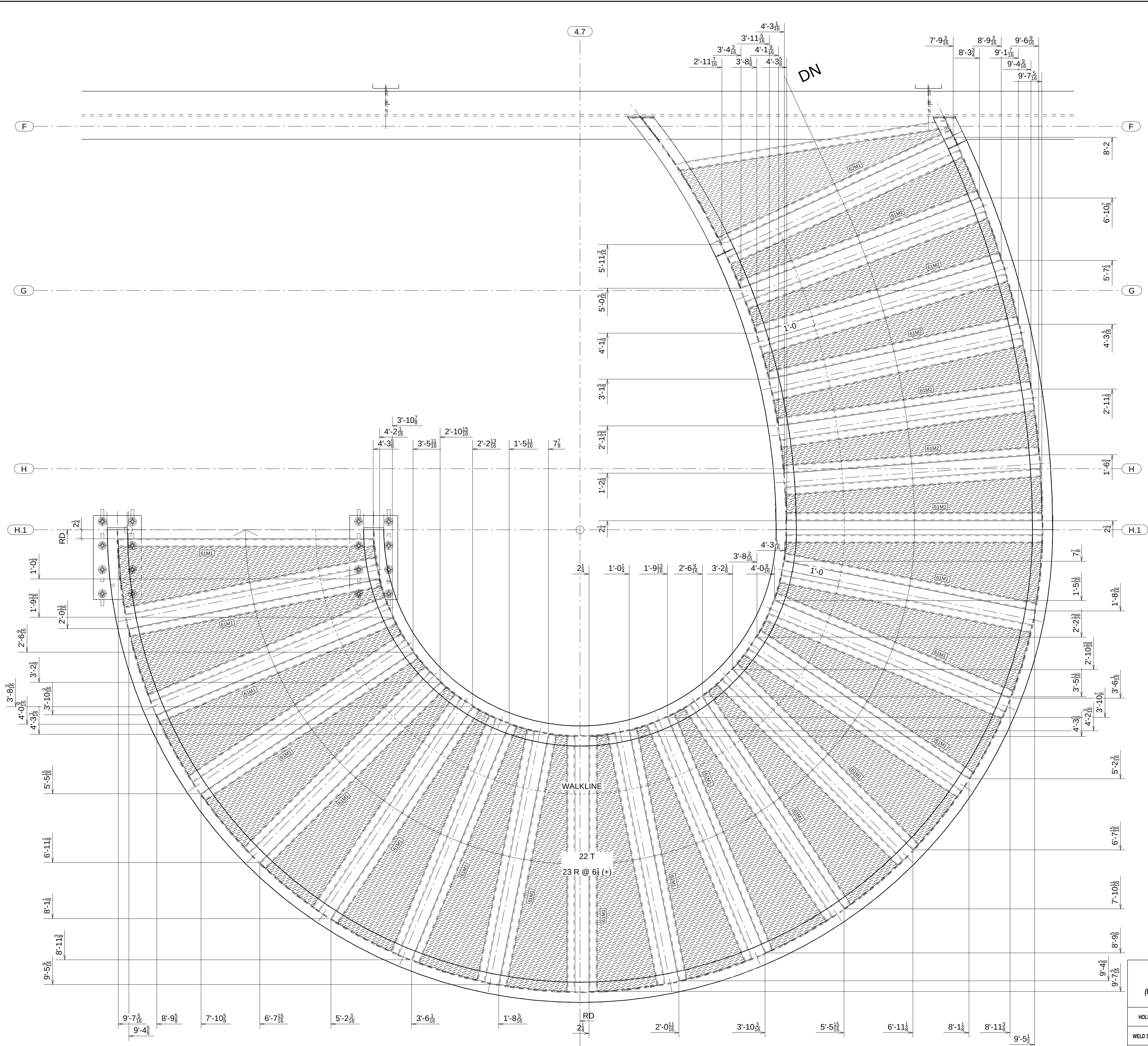
TREAD LAYOUT PLAN
