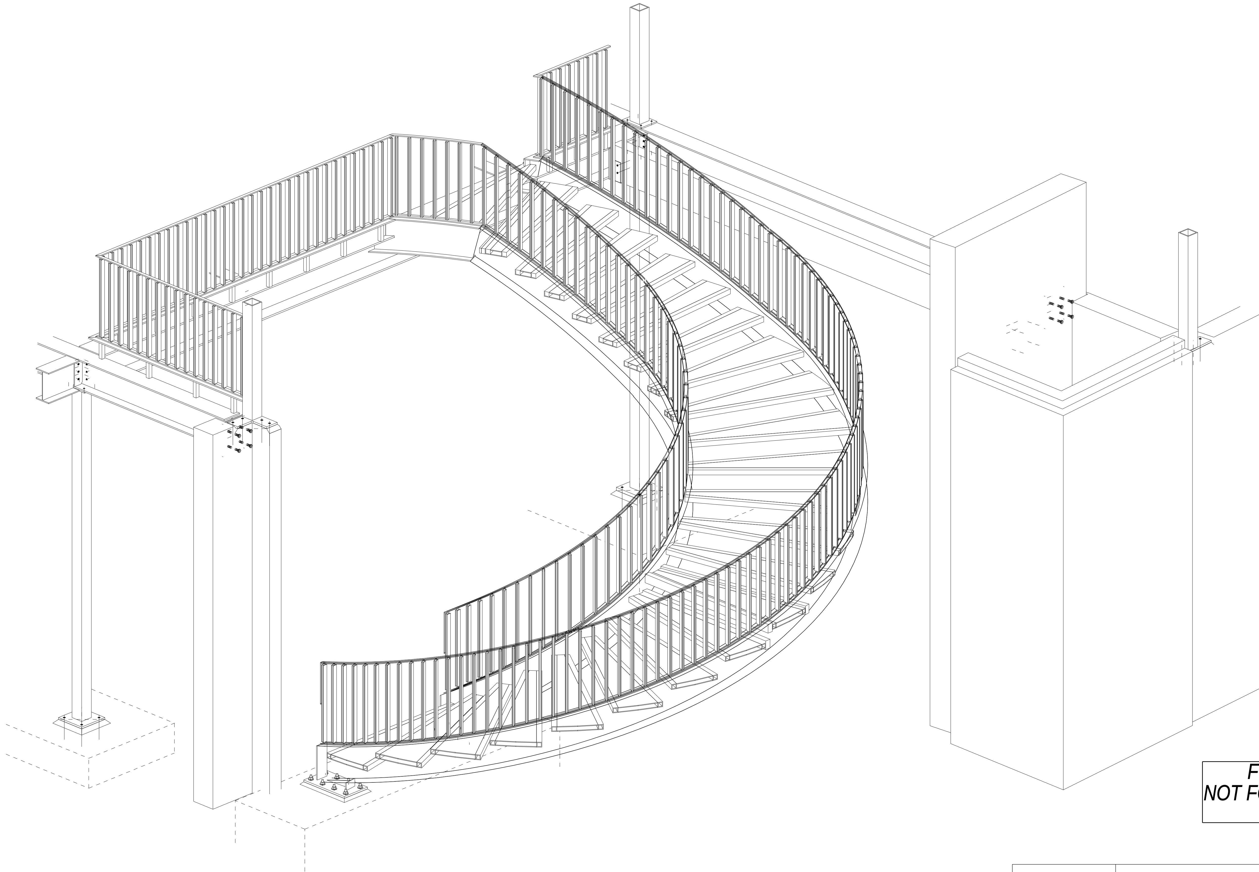
STAIR - 3D VIEW LOOKING NORTHEAST
