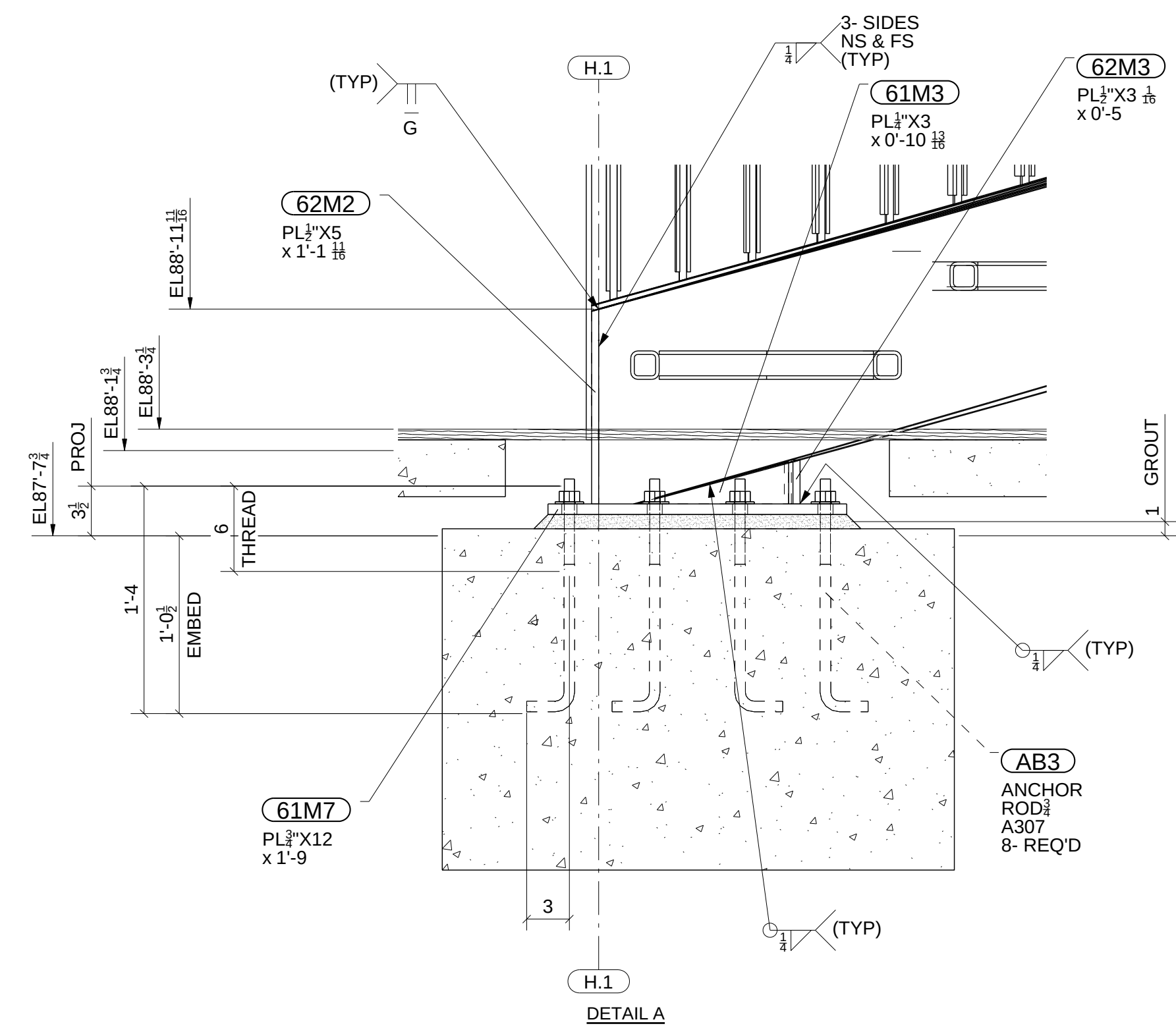
DETAIL A
