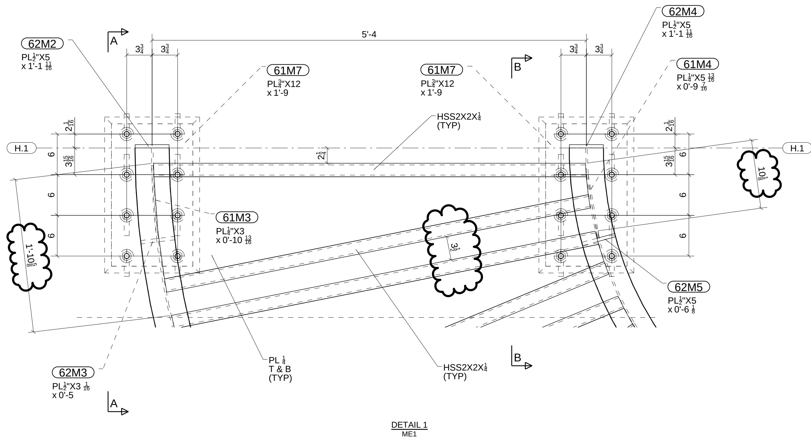
DETAIL 1 ME1
