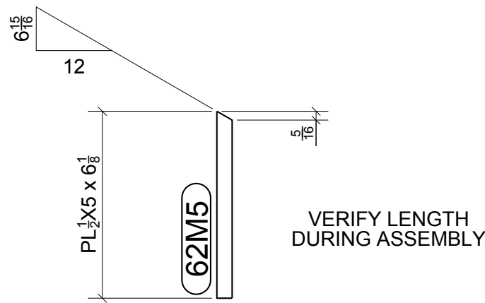
ONE - END PLATE - 62M5
