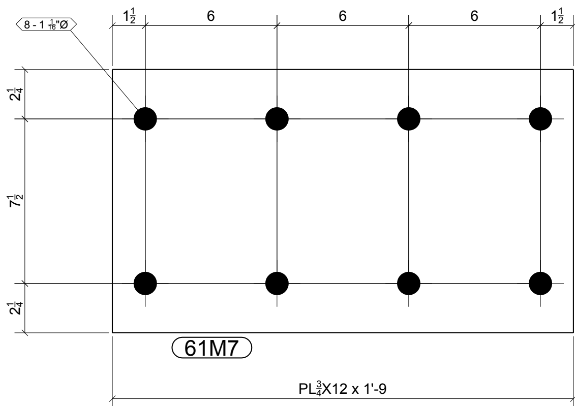
2 - PLATES - 61M7
