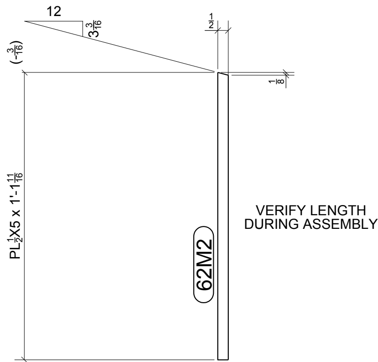
ONE - END PLATE - 62M2
