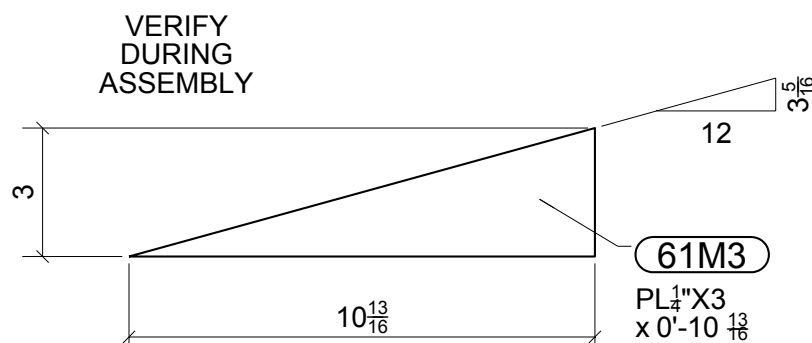
ONE - PLATE - 61M3
