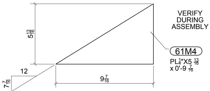
ONE - PLATE - 61M4
