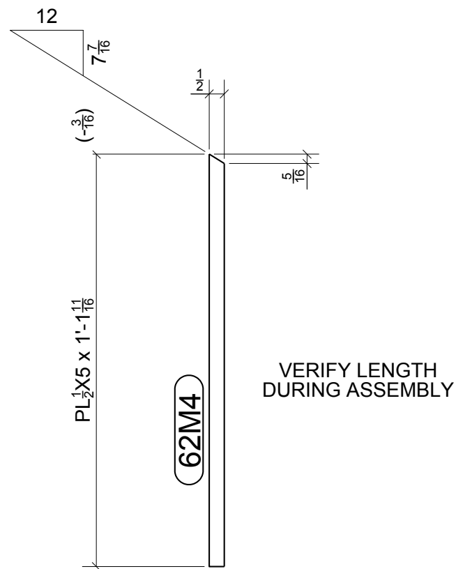
ONE - END PLATE - 62M4
