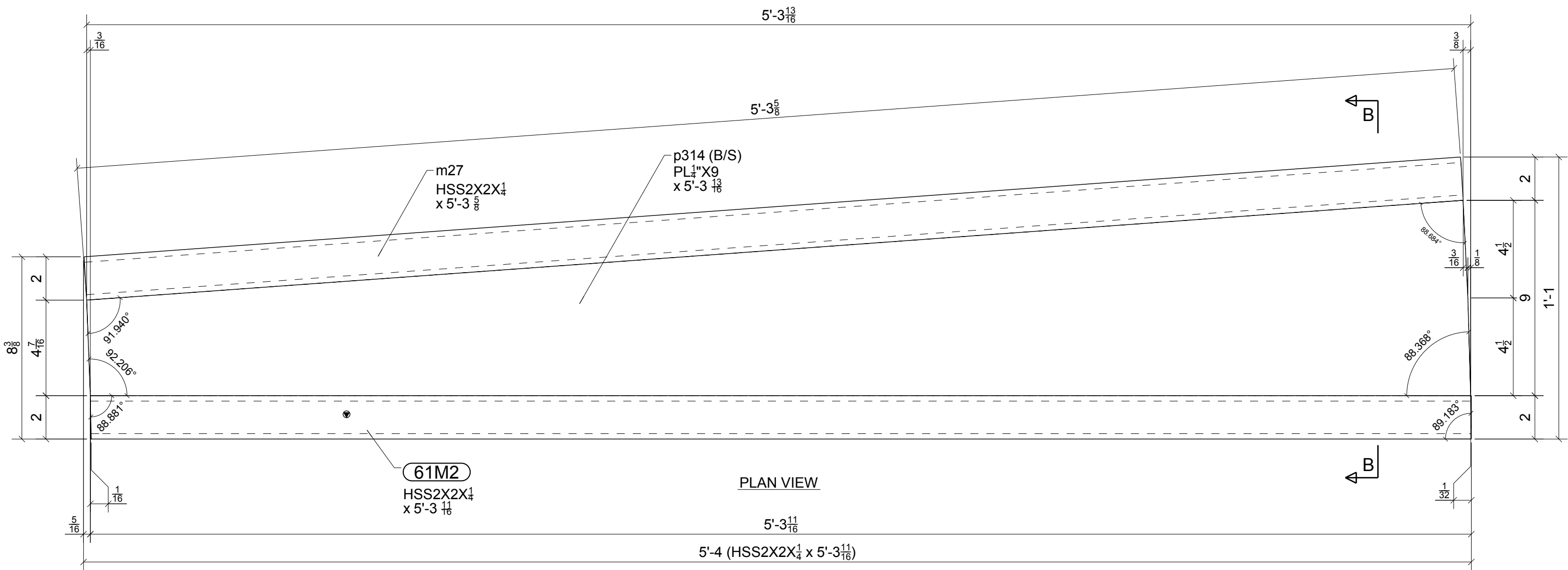
6 - TREAD SUPPORTS - 61M2
