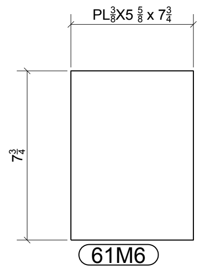
ONE - PLATE - 61M6
