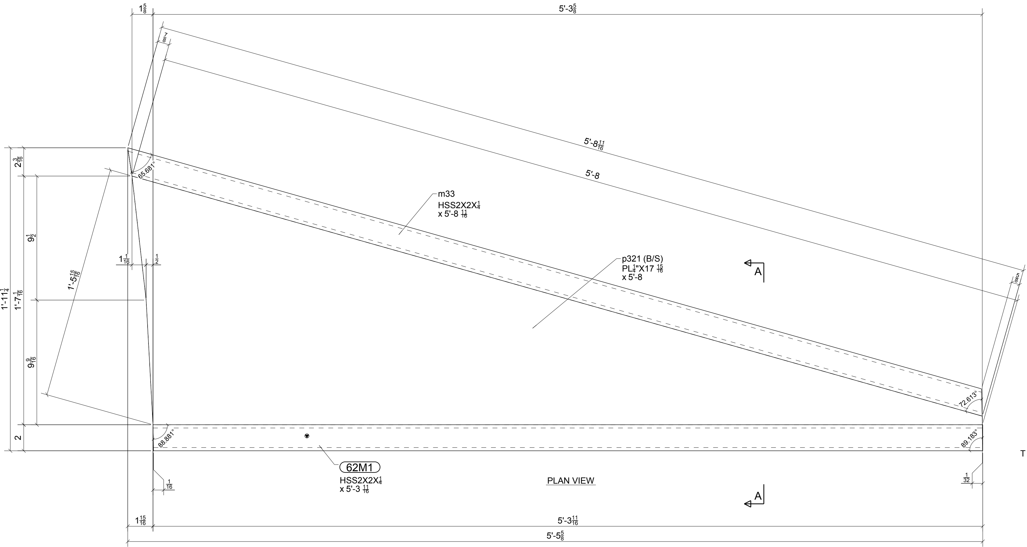
ONE - TREAD SUPPORT - 62M1
