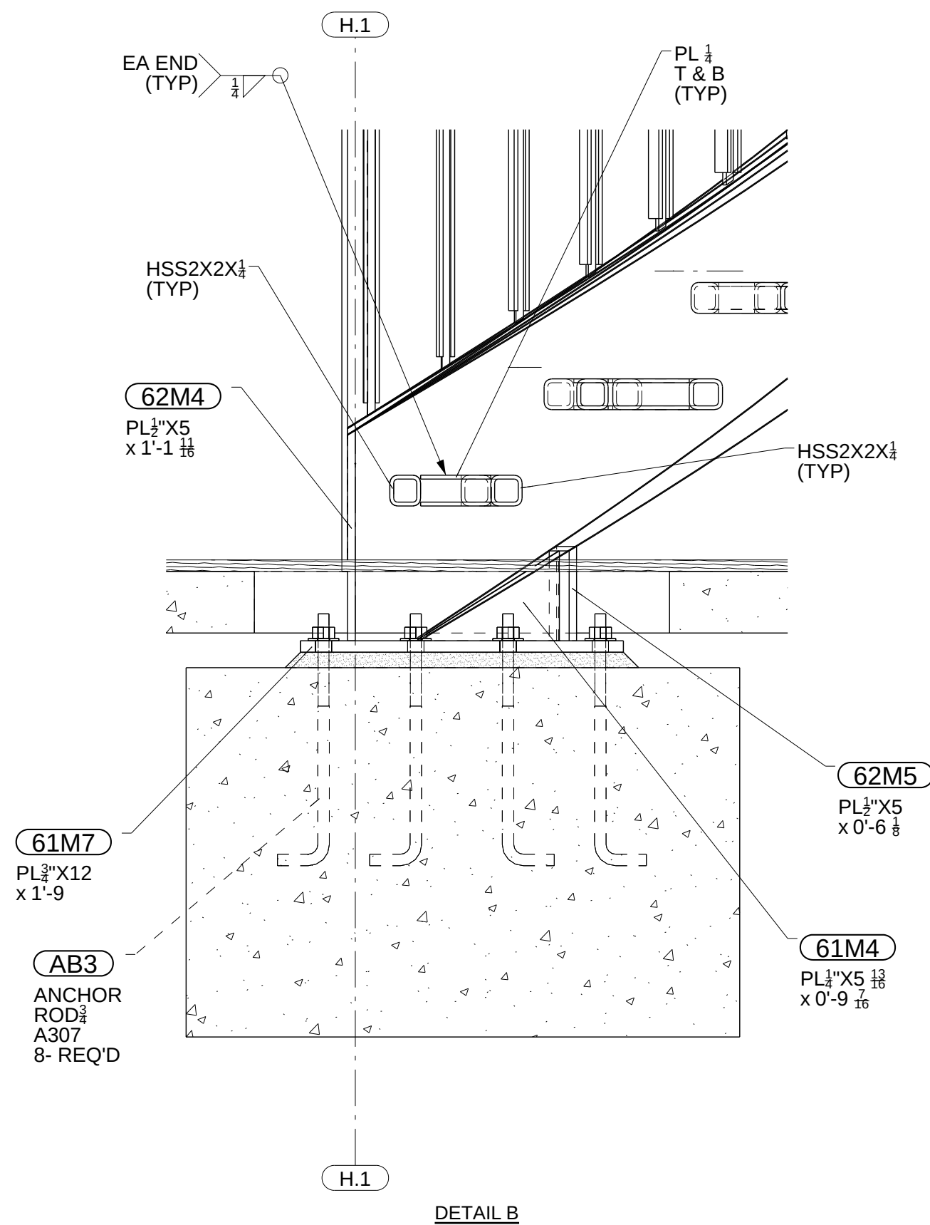
DETAIL B
