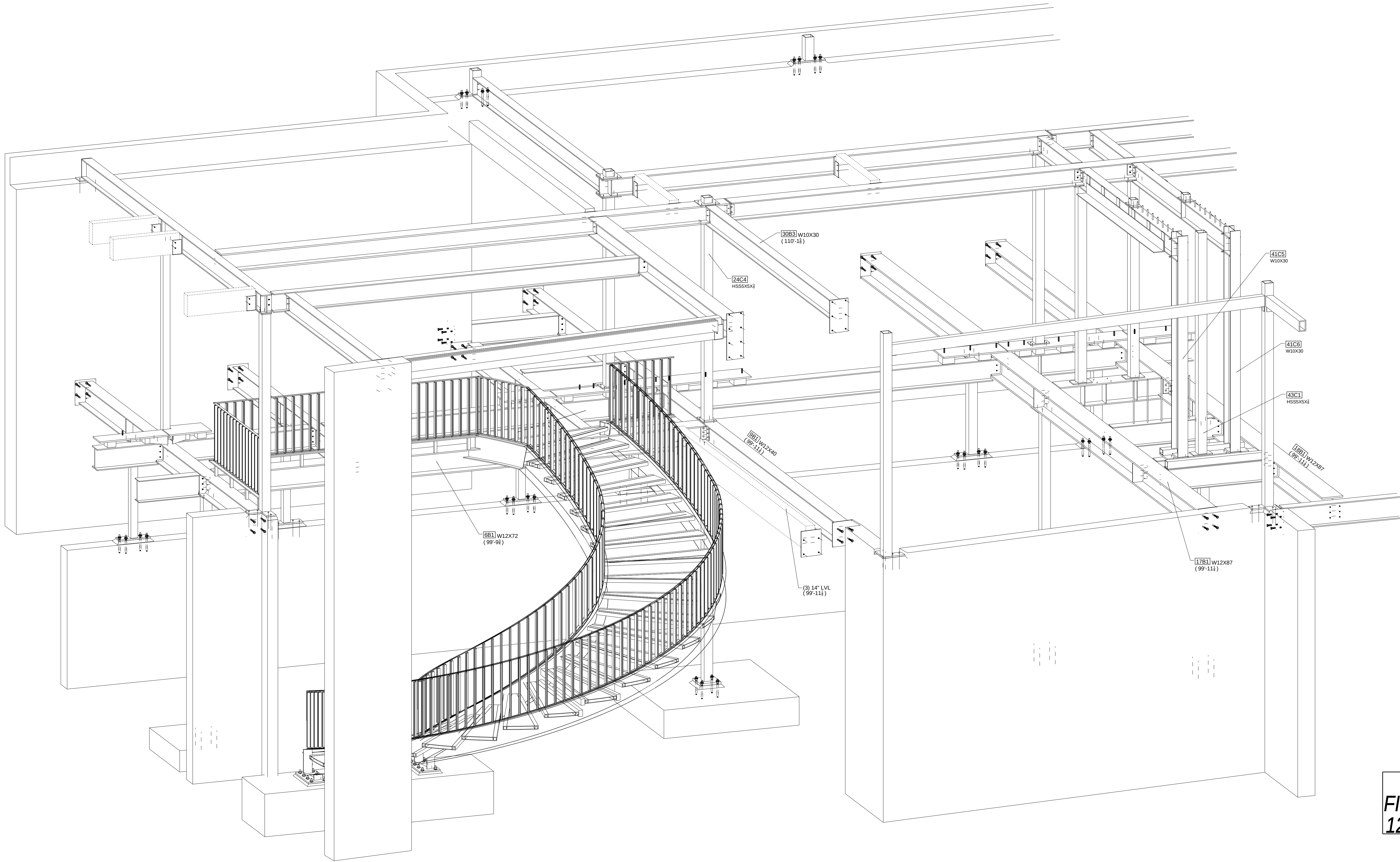
3D VIEW ERECTION FRAMING
