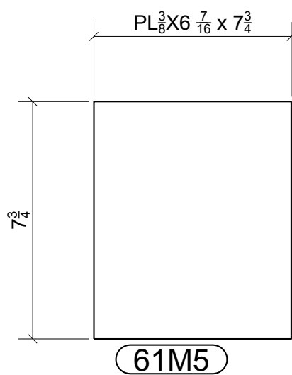
ONE - PLATE - 61M5
